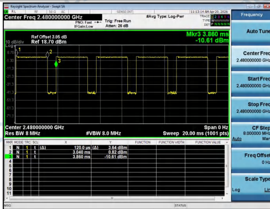
Duty_Cycle_NVNT_ANT1_3-DH5_2480
