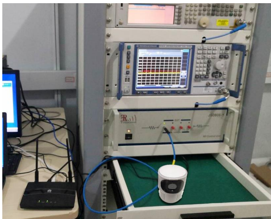
1.3. Photo of DFS Measurement
