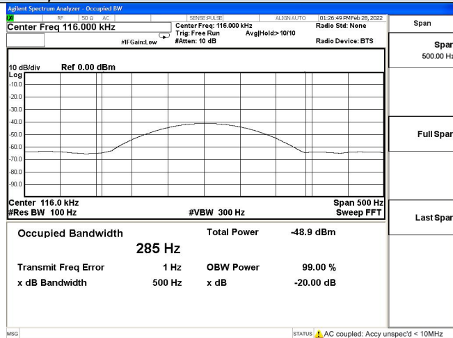
Test plot of 99% and 20 dB Bandwidth Measurement
