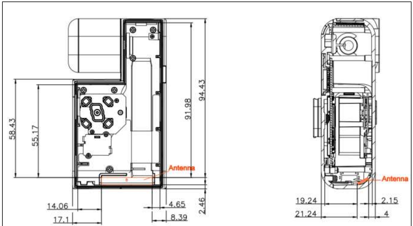
Figure F-1 Antenna Location
