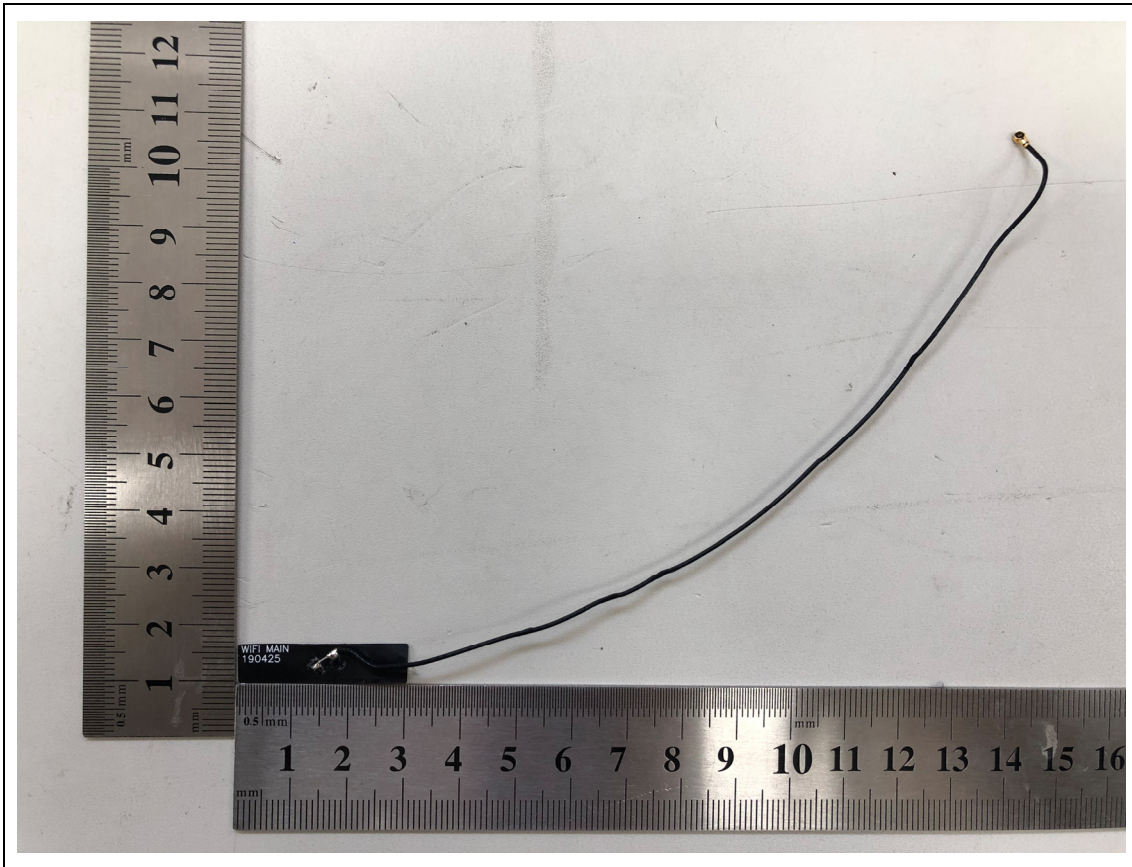
<WLAN Main Antenna>
