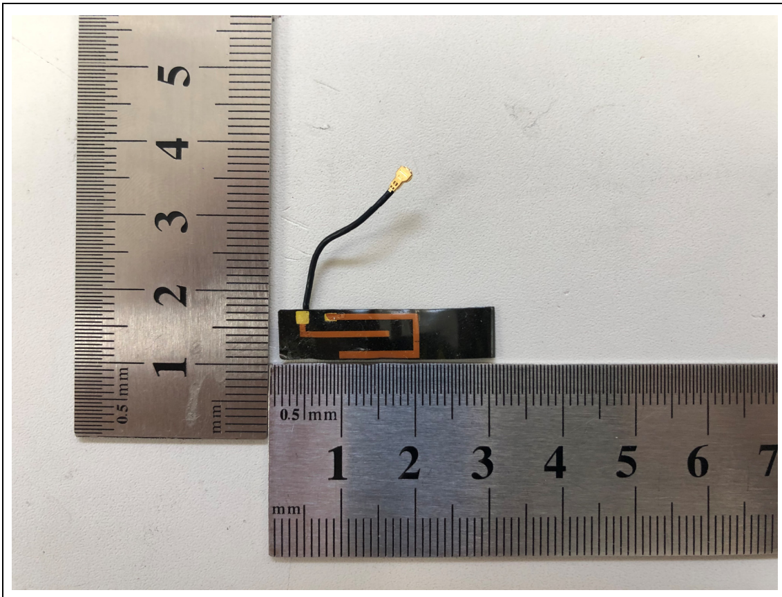
< WLAN Sub Antenna >
