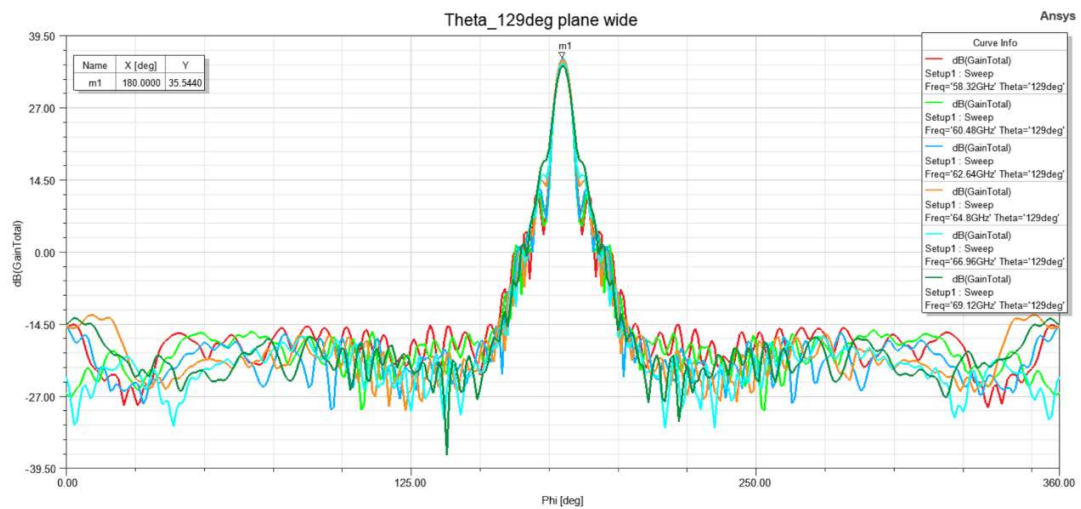
Figure 3: Peak Antenna gain wide view
