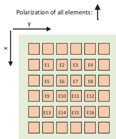
Figure 4: Diagram of the 16-element Radio Module for Reflector
