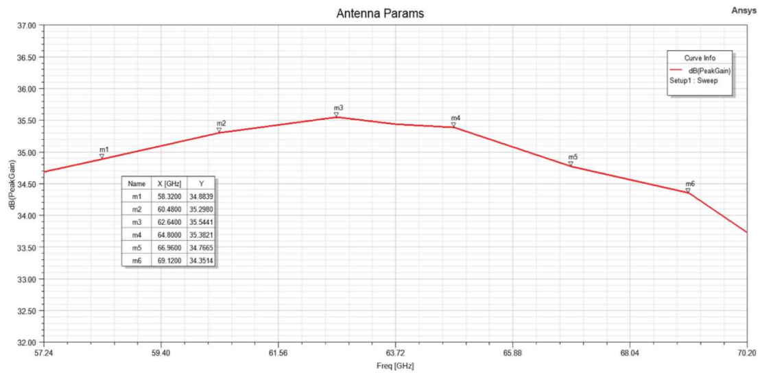
Figure 2: Peak Antenna gains across all channels
