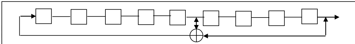
Linier Feedback Shift Register for Generator of the PRBS sequence
