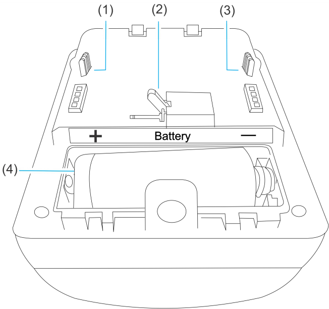
Figure 2: Sensor pins and tamper switch
