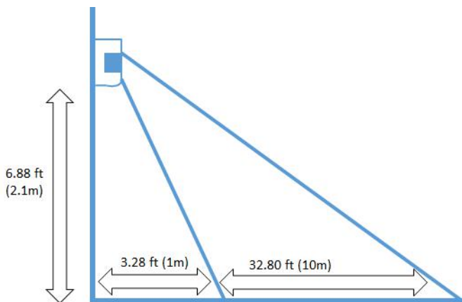
Figure 1: Sensor range and detection
