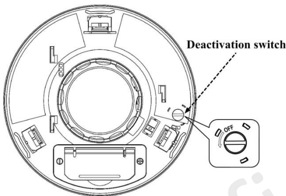
Figure12: Location of deactivation switch for model
