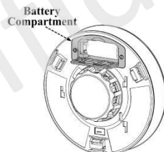
Figure 8: Battery compartment
