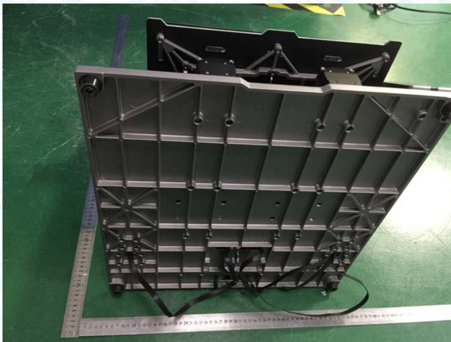
Photo 6 Appearance of EUT (Model: 80013)
