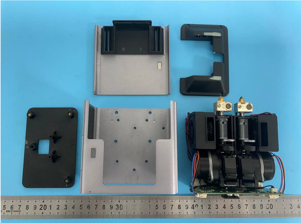
3DP Module (TH-F-DUAL-AS ,TH-F-DUAL-MS)
