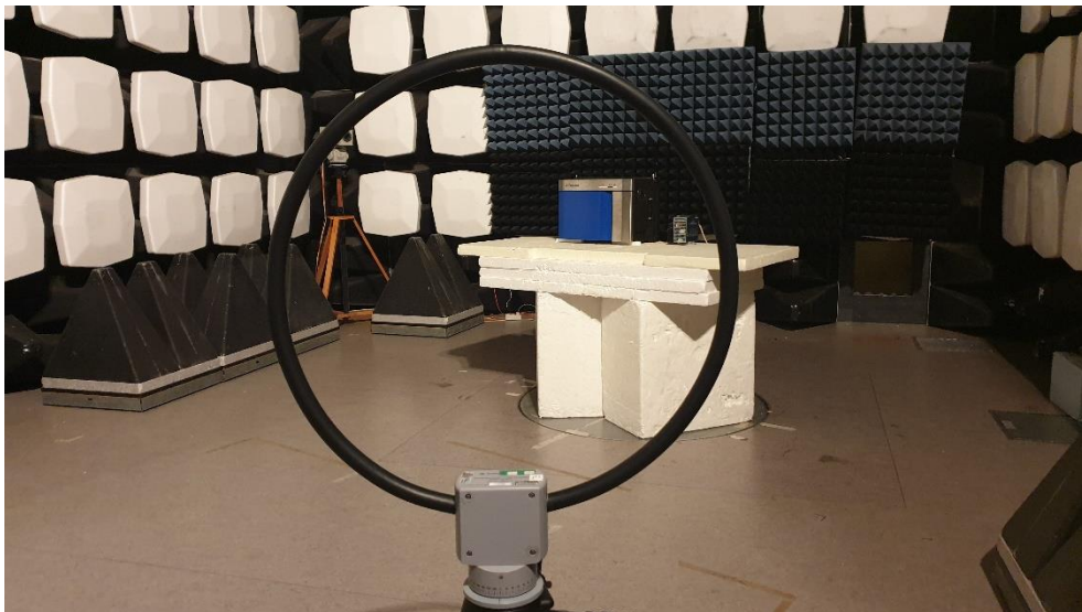
Photo 6. Radiated emission test setup in SAC. 9 kHz – 30 MHz.
