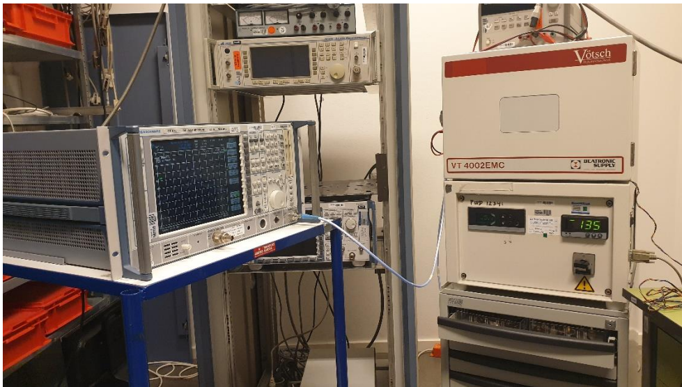
Photo 4. Frequency stability under temperature variation test set up. Occupied bandwidth -20 dB test set up.
