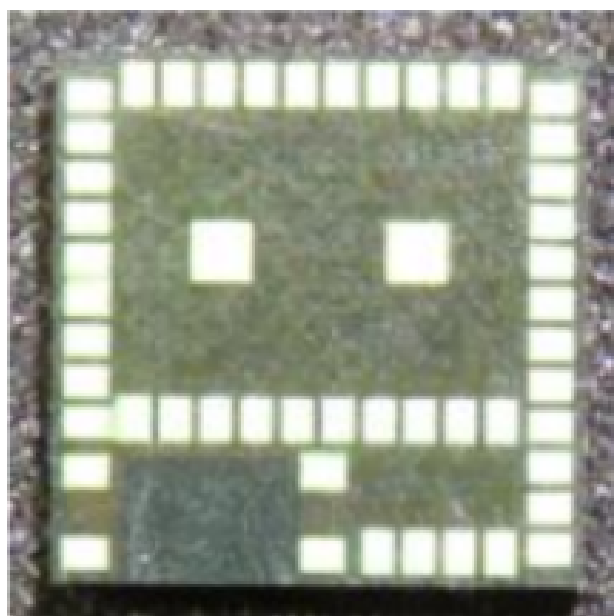
Figure 2: Bottom view
