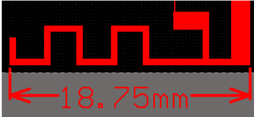
Figure 1 - Antenna structure.
