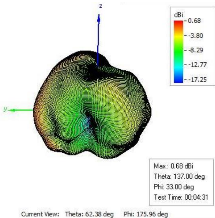
Figure 2 - 3D gain.
