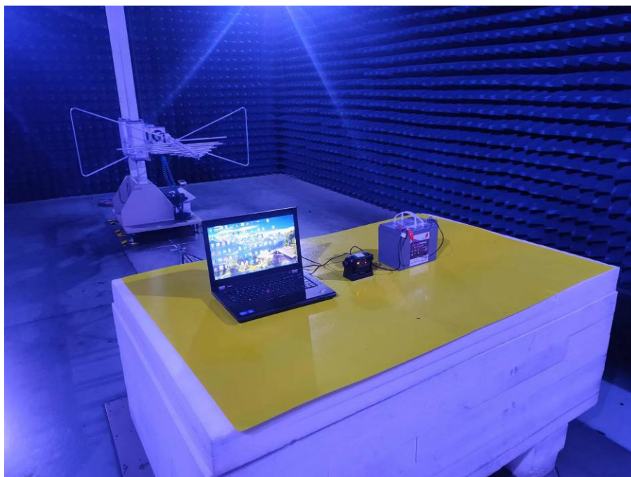
Photo of Radiated Emission Measurement (Below 1G) - DC Power Supply Port
