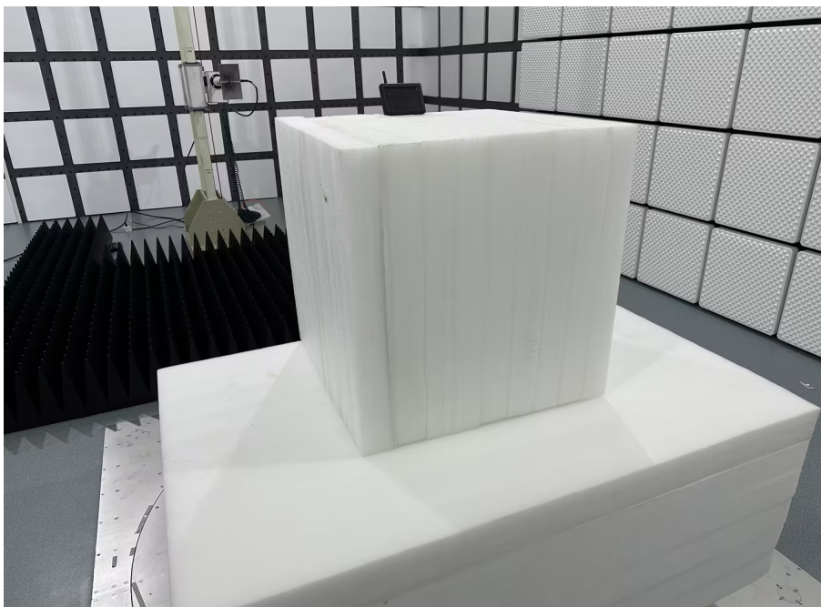
Photo of Radiated Emission Measurement (Above 1G)
