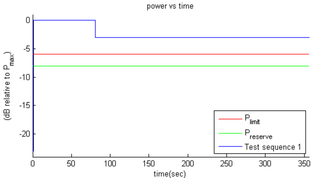
Figure 10-1 Test sequence 1 waveform
