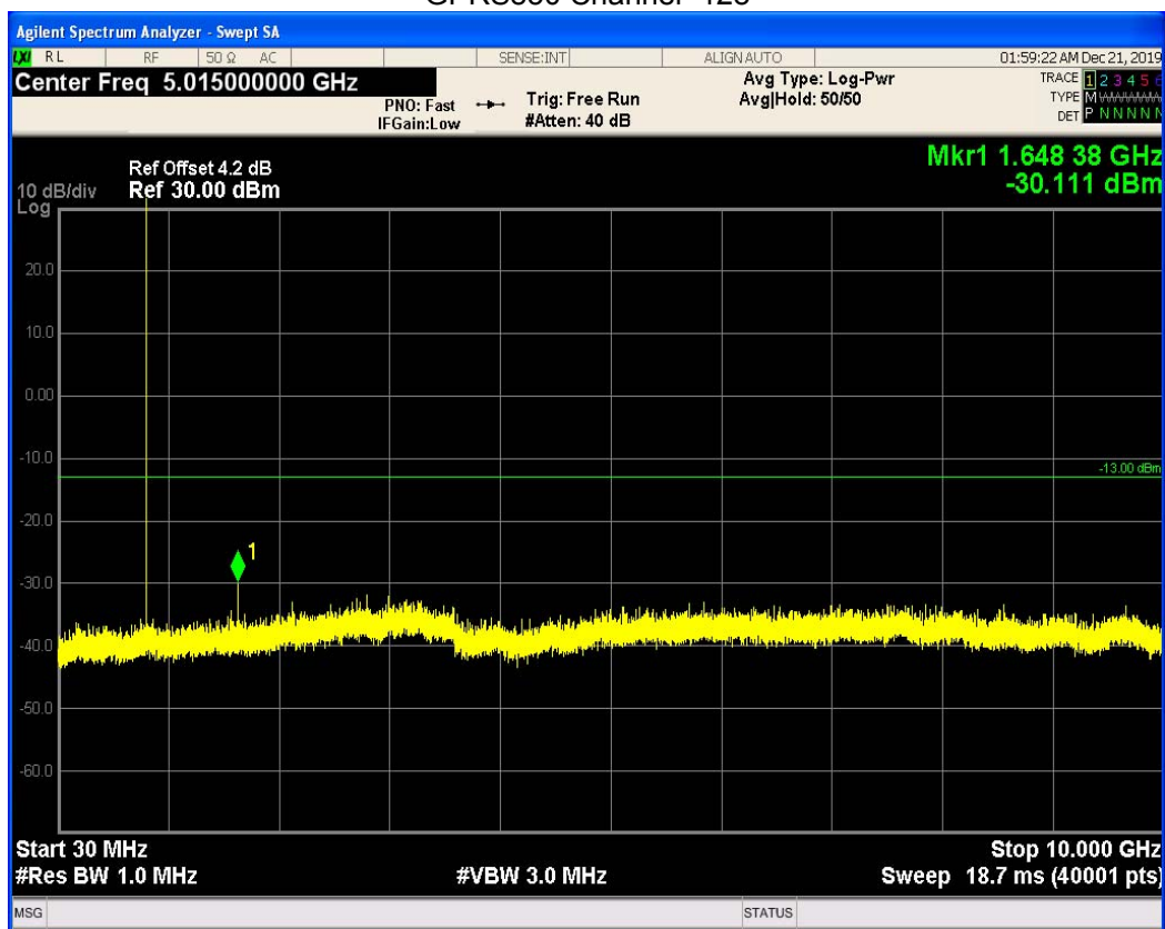
GPRS850 Channel=128
