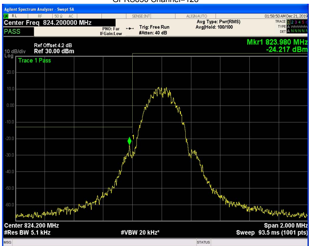
GPRS850 Channel=128
