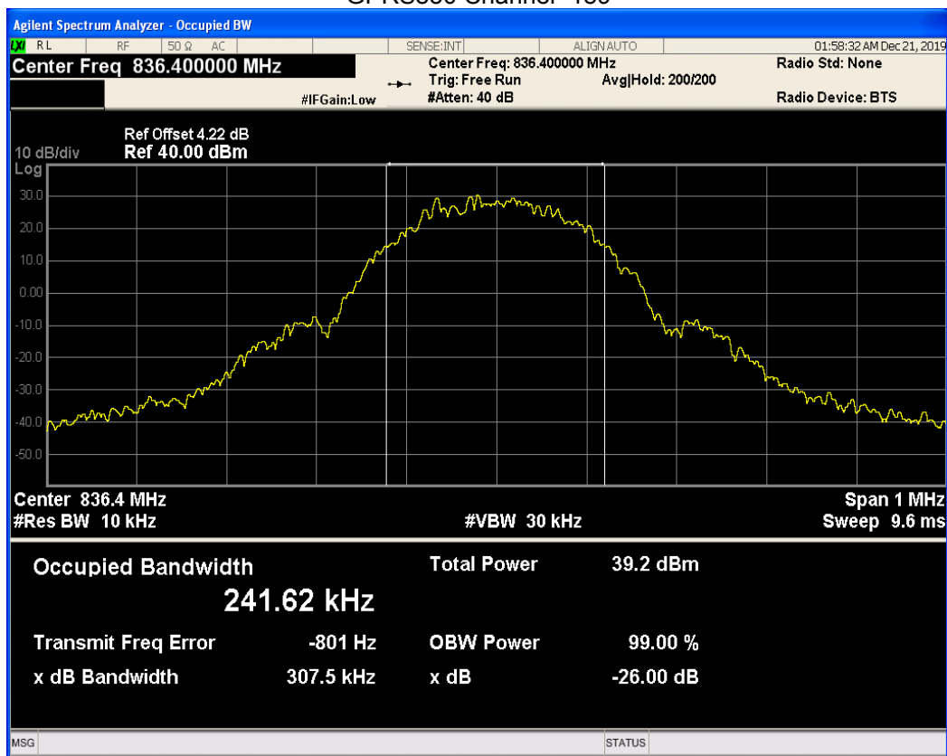
GPRS850 Channel=189
