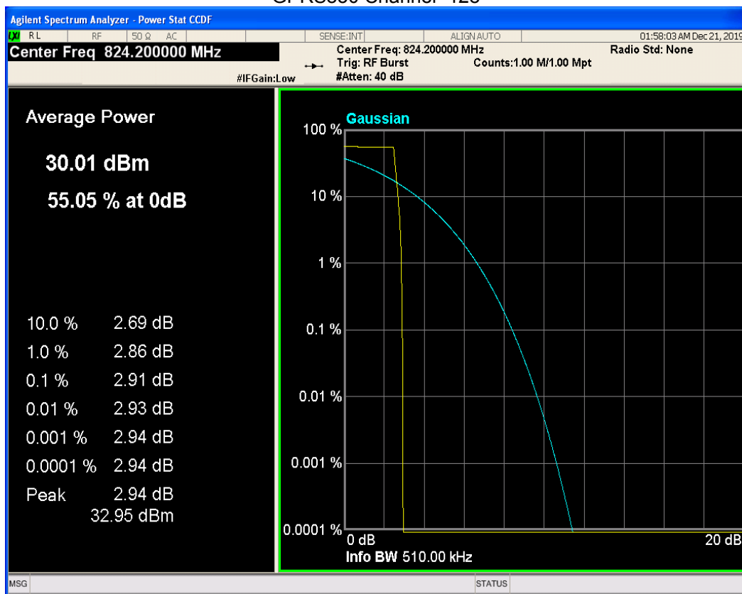
GPRS850 Channel=128
