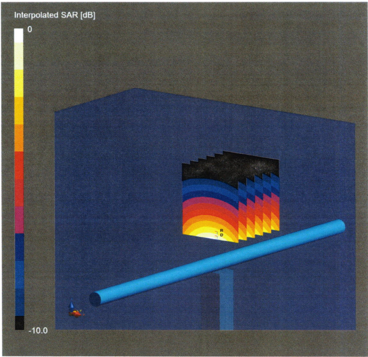
0 dB = 3.30 W/Kg
