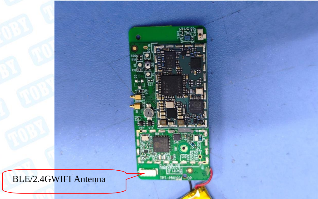
Photo 17 Appearance of PCB
