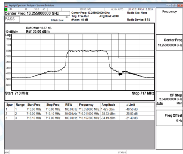
Band12-3MHz-16QAM-23165-6-0-High-716.16--34.49-21.49-PASS
