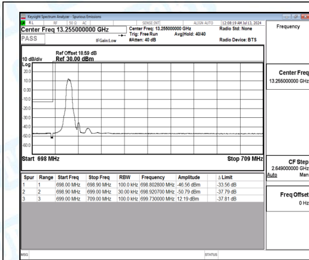
Band12-10MHz-16QAM-23060-1-0-Low-698.80--46.56-33.56-PASS
