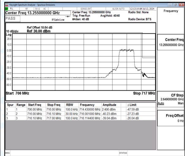
Band12-10MHz-16QAM-23130-6-0-High-716.11--39.04-26.04-PASS
