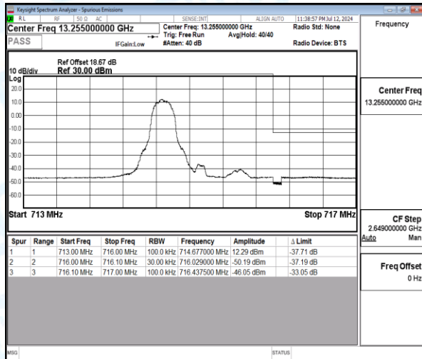
Band12-3MHz-QPSK-23165-1-0-High-716.44--46.05-33.05-PASS
