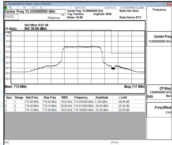
Band12-3MHz-QPSK-23165-6-0-High-716.18--35.09-22.09-PASS
