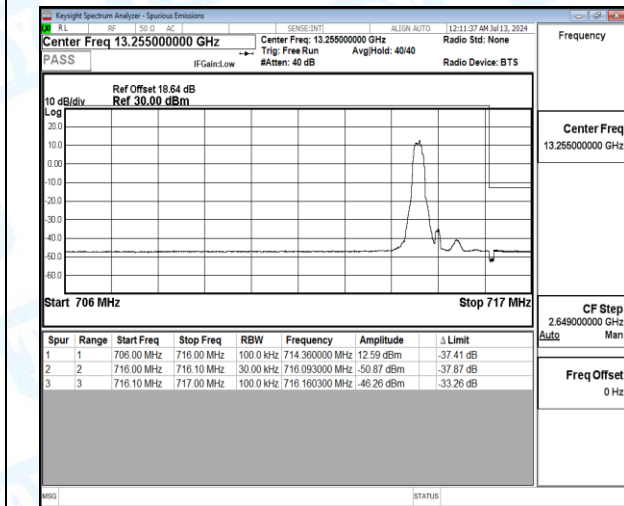
Band12-10MHz-16QAM-23130-1-0-High-716.16--46.26-33.26-PASS
