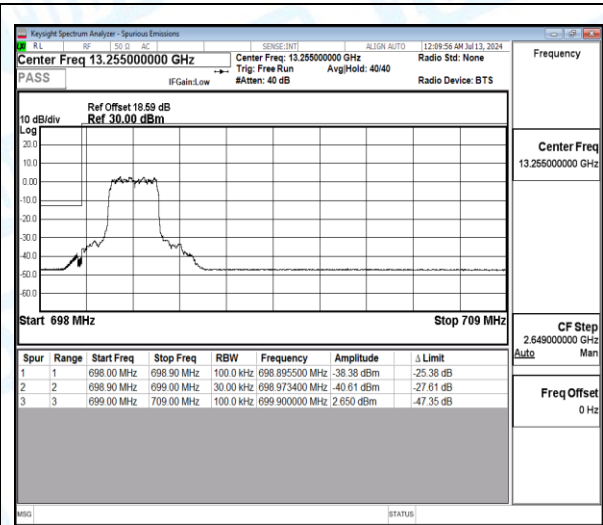
Band12-10MHz-16QAM-23060-6-0-Low-698.90--38.38-25.38-PASS
