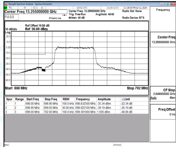
Band12-3MHz-16QAM-23025-6-0-Low-698.83--35.34-22.34-PASS
