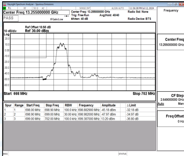
Band12-3MHz-16QAM-23025-1-0-Low-698.88--45.18-32.18-PASS
