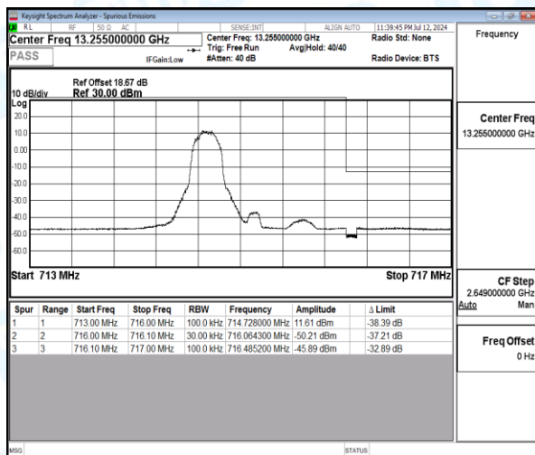
Band12-3MHz-16QAM-23165-1-0-High-716.49--45.89-32.89-PASS
