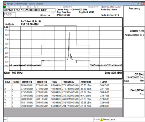
Band13-10MHz-QPSK-23230-1-0-High-794.78--55.64-20.64-PASS
