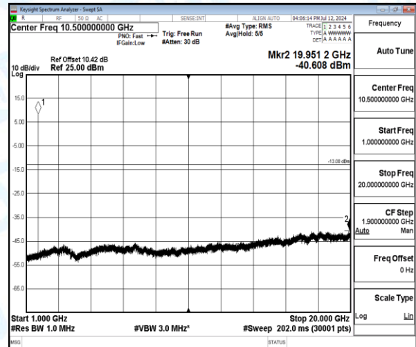
Band4-1.4MHz-QPSK-19957-1-0-Low-1000-20000-19951.23--40.61-27.61--13-PASS
