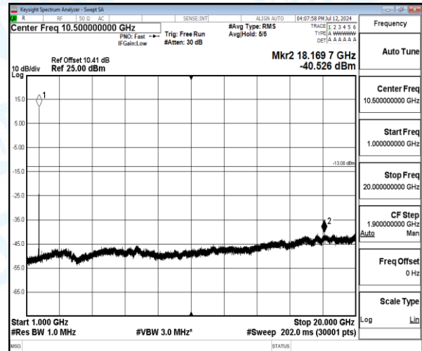
Band4-1.4MHz-16QAM-20175-1-0-Low-1000-20000-18169.67--40.53-27.53--13-PASS
