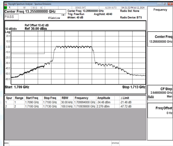
Band4-3MHz-16QAM-19965-6-0-Low-1709.99--34.48-21.48-PASS
