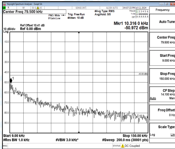
Band4-1.4MHz-16QAM-20175-1-0-Low-0.009-0.15-0.01--50.97-7.97--43-PASS
