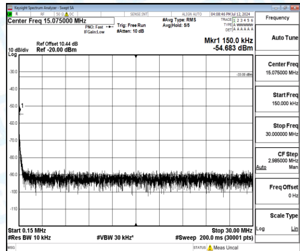
Band4-1.4MHz-16QAM-20393-1-0-High-0.15-30-0.15--54.68-21.68--33-PASS
