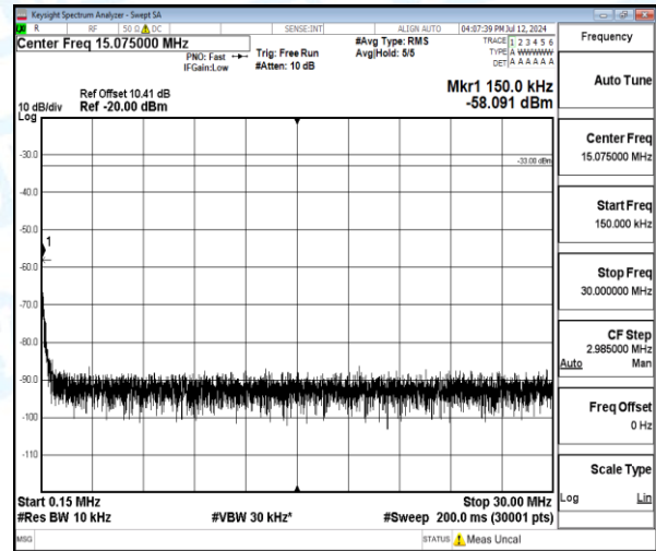
Band4-1.4MHz-16QAM-20175-1-0-Low-0.15-30-0.15--58.09-25.09--33-PASS
