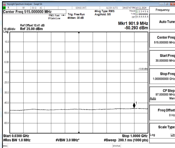
Band4-1.4MHz-16QAM-20175-1-0-Low-30-1000-901.93--50.29-37.29--13-PASS
