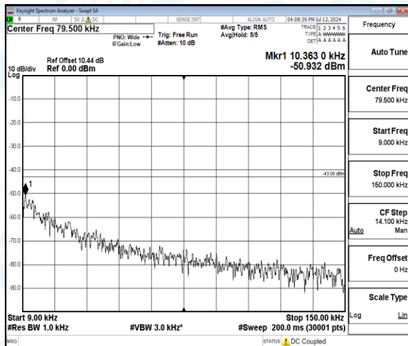
Band4-1.4MHz-16QAM-20393-1-0-High-0.009-0.15-0.01--50.93-7.93--43-PASS
