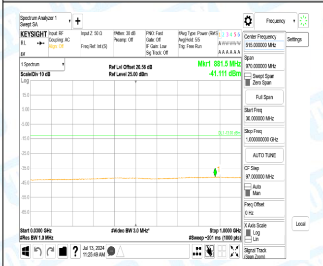
Band4-3MHz-16QAM-20175-1-0-Low-30-1000-881.54--41.11-28.11--13-PASS
