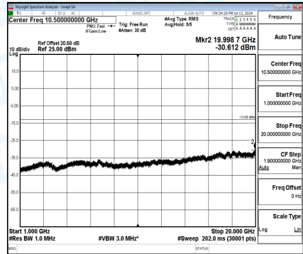
Band4-10MHz-QPSK-20350-1-0-High-1000-19998.73--30.61-17.61--13-PASS
