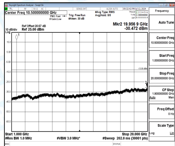
Band4-10MHz-16QAM-20000-1-0-Low-1000-20000-19956.93--30.47-17.47--13-PASS
