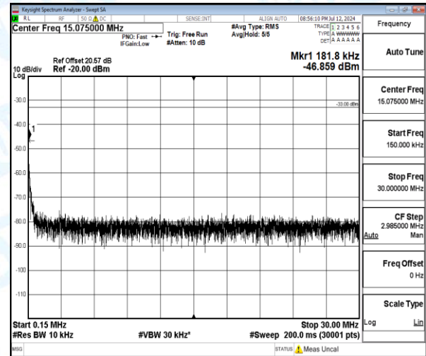
Band4-5MHz-16QAM-19975-1-0-Low-0.15-30-0.18--46.86-13.86--33-PASS
