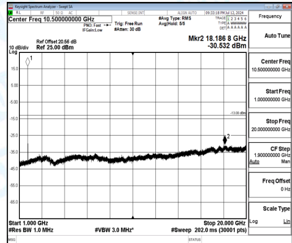
Band4-10MHz-QPSK-20175-1-0-Low-1000-20000-18186.77--30.53-17.53--13-PASS
