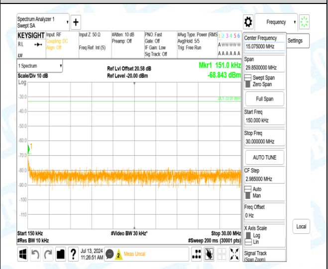
Band4-3MHz-16QAM-20385-1-0-High-0.15-30-0.15--68.84-35.84--33-PASS
