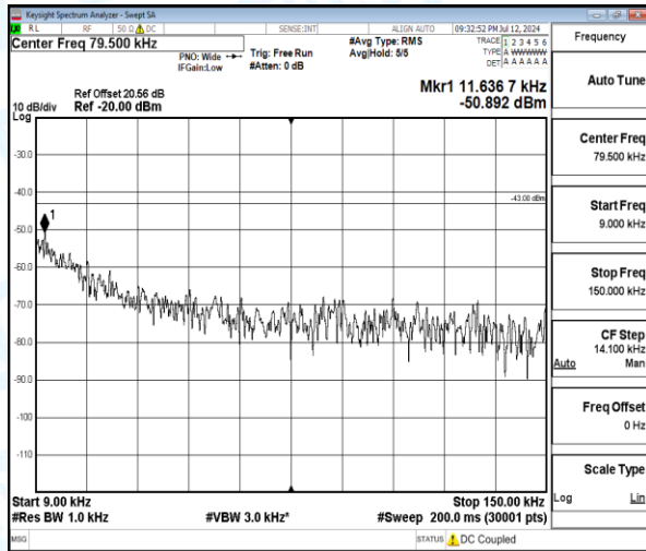
Band4-10MHz-QPSK-20175-1-0-Low-0.009-0.15-0.01--50.89-7.89--43-PASS
