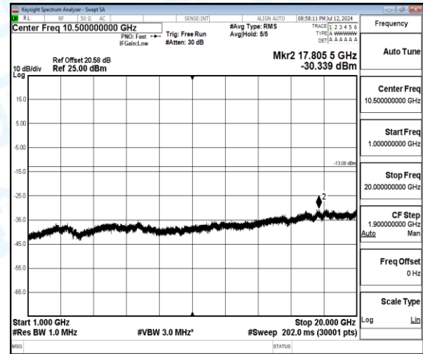
Band4-5MHz-QPSK-20375-1-0-High-1000-20000-17805.5--30.34-17.34--13-PASS
