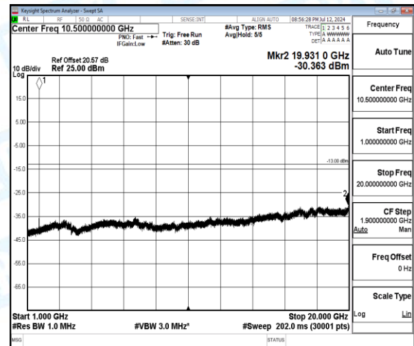
Band4-5MHz-16QAM-19975-1-0-Low-1000-20000-19930.97--30.36-17.36--13-PASS
