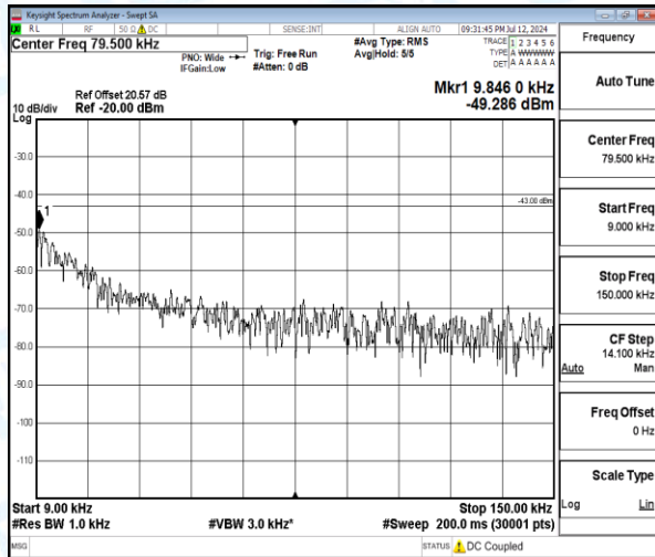
Band4-10MHz-QPSK-20000-1-0-Low-0.009-0.15-0.01--49.29-6.29--43-PASS
