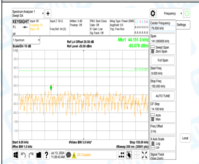
Band4-3MHz-16QAM-20385-1-0-High-0.009-0.15-0.04--65.08-22.08--43-PASS
