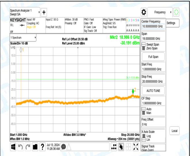
Band4-3MHz-QPSK-20385-1-0-High-1000-20000-18986.03--30.19-17.19--13-PASS
