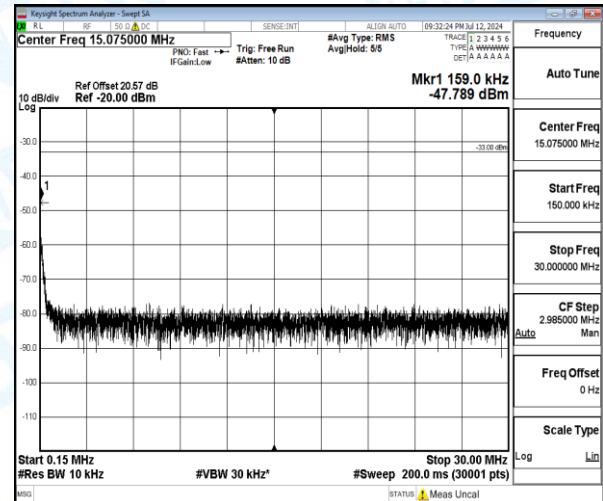
Band4-10MHz-16QAM-20000-1-0-Low-0.15-30-0.16--47.79-14.79--33-PASS
