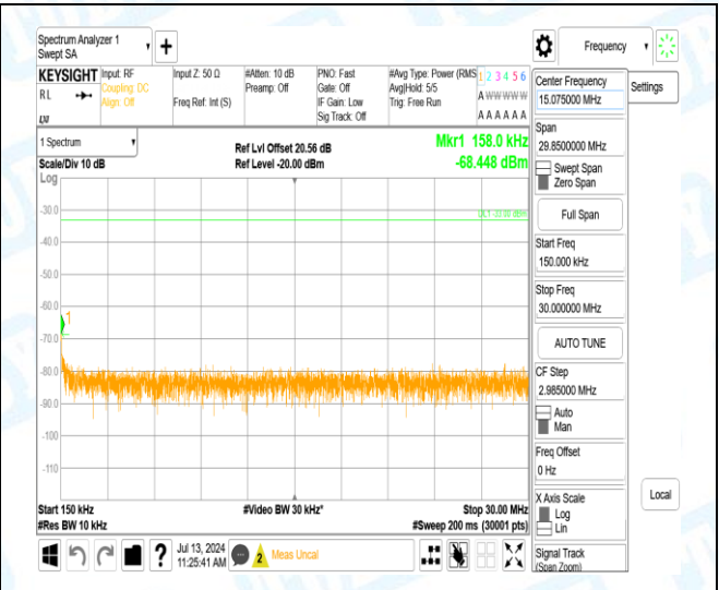
Band4-3MHz-16QAM-20175-1-0-Low-0.15-30-0.16--68.45-35.45--33-PASS
