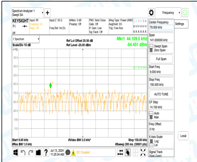
Band4-3MHz-16QAM-20175-1-0-Low-0.009-0.15-0.04--64.45-21.45--43-PASS
