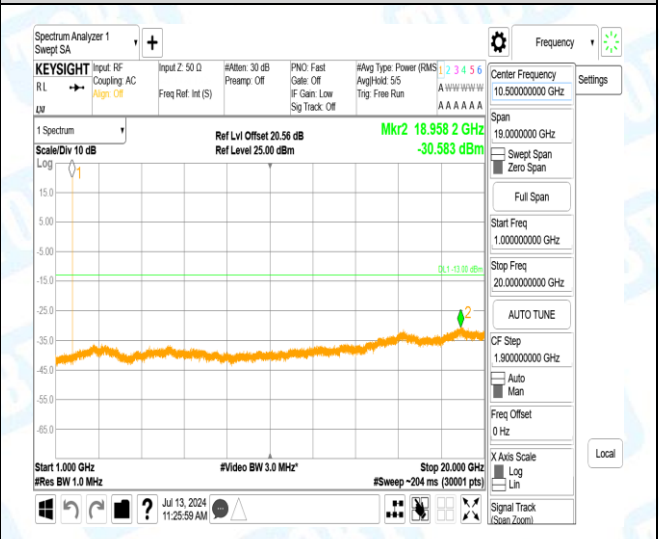
Band4-3MHz-16QAM-20175-1-0-Low-1000-20000-18958.17--30.58-17.58--13-PASS
