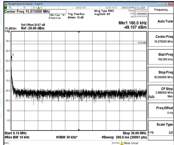
Band4-5MHz-QPSK-19975-1-0-Low-0.15-30-0.16--49.11-16.11--33-PASS
