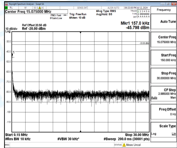
Band4-10MHz-QPSK-20175-1-0-Low-0.15-30-0.16--45.8-12.8--33-PASS
