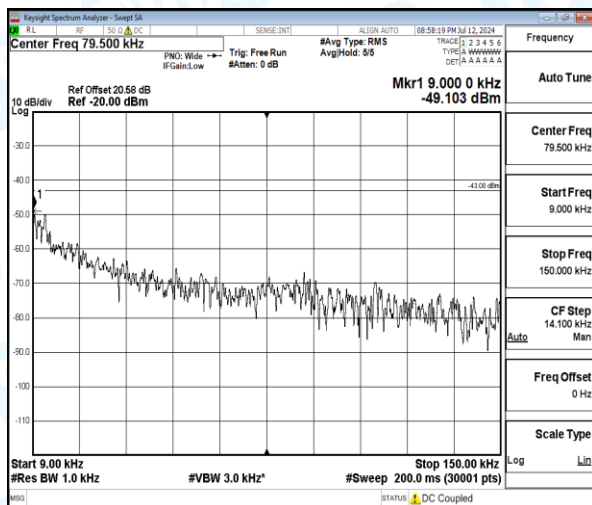
Band4-5MHz-16QAM-20375-1-0-High-0.09-0.15-0.01--49.1-6.1--43-PASS
