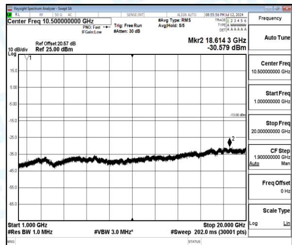
Band4-5MHz-QPSK-19975-1-0-Low-1000-20000-18614.27--30.58-17.58--13-PASS
