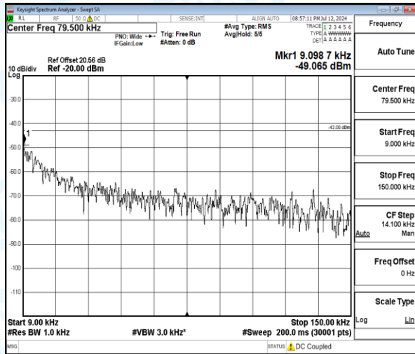
Band4-5MHz-16QAM-20175-1-0-Low-0.09-0.15-0.01--49.07-6.07--43-PASS
