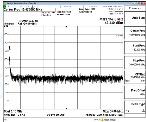
Band4-10MHz-QPSK-20000-1-0-Low-0.15-30-0.16--48.44-15.44--33-PASS
