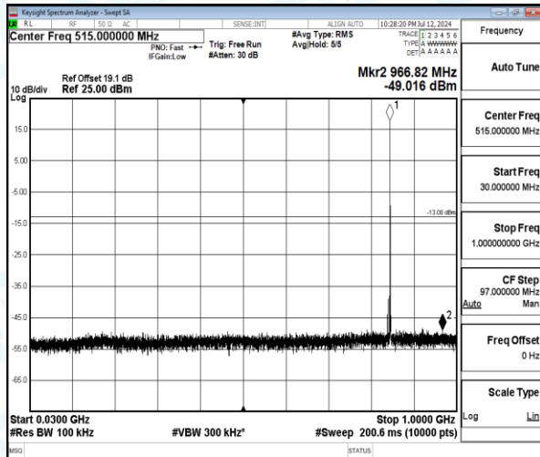
Band5-1.4MHz-16QAM-20643-1-0-High-30-1000-966.82--49.02-36.02--13-PASS
