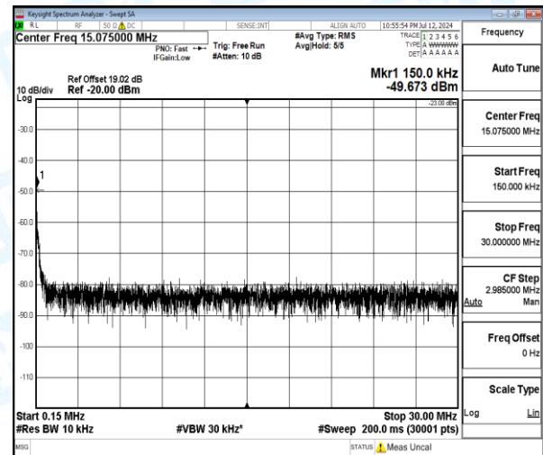
Band5-5MHz-16QAM-20425-1-0-Low-0.15-30-0.15--49.67-26.67--23-PASS
