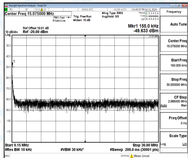
Band5-3MHz-16QAM-20415-1-0-Low-0.15-30-0.15--49.63-26.63--23-PASS
