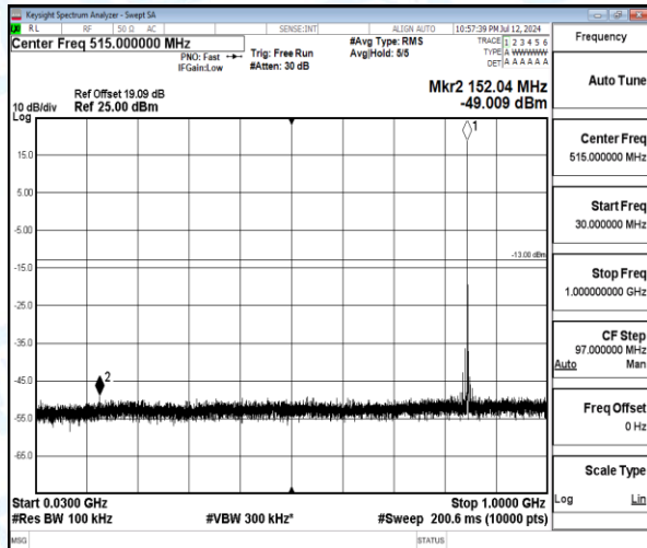
Band5-5MHz-QPSK-20625-1-0-High-30-1000-152.04--49.01-36.01--13-PASS
