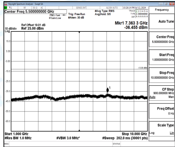
Band5-1.4MHz-16QAM-20407-1-0-Low-1000-10000-7363.3--36.46-23.46--13-PASS
