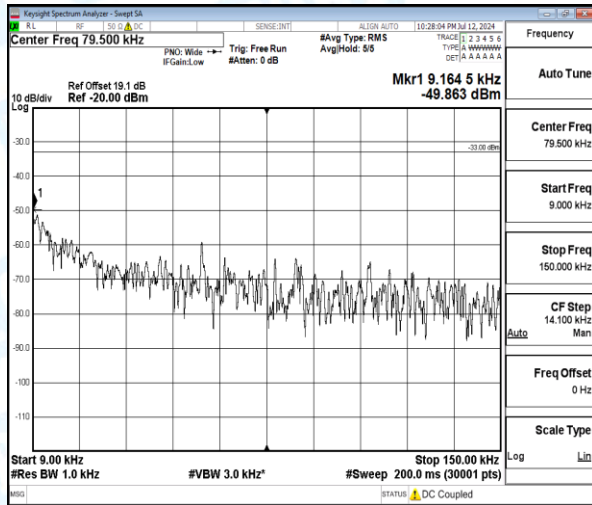
Band5-1.4MHz-16QAM-20643-1-0-High-0.009-0.15-0.01--49.86-16.86--33-PASS
