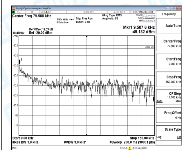
Band5-10MHz-QPSK-20450-1-0-Low-0.009-0.15-0.01--49.13-16.13--33-PASS
