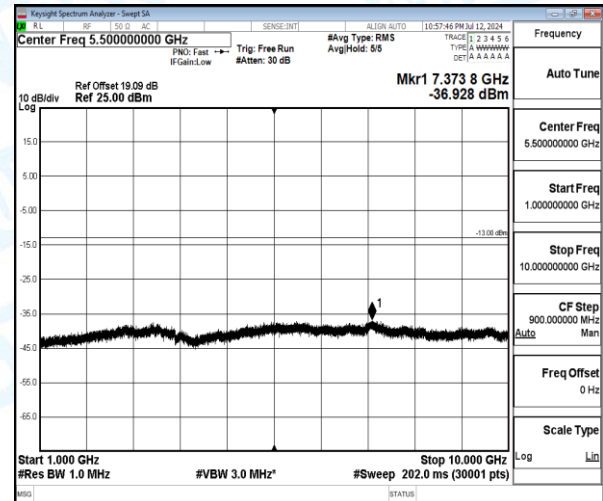
Band5-5MHz-QPSK-20625-1-0-High-1000-10000-7373.8--36.93-23.93--13-PASS
