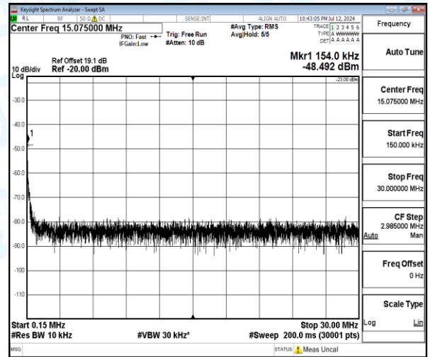
Band5-3MHz-16QAM-20635-1-0-High-0.15-30-0.15--48.49-25.49--23-PASS
