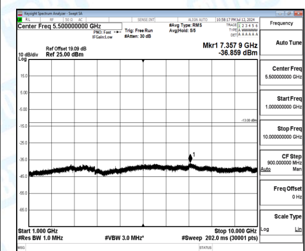
Band5-5MHz-16QAM-20625-1-0-High-1000-10000-7357.9--36.86-23.86--13-PASS
