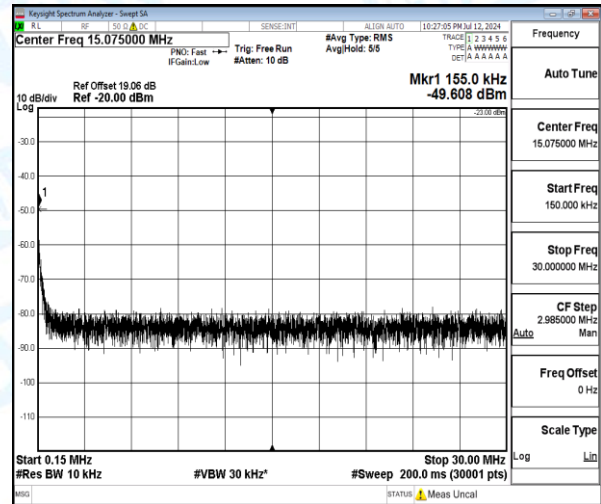
Band5-1.4MHz-16QAM-20525-1-0-Low-0.15-30-0.15--49.61-26.61--23-PASS
