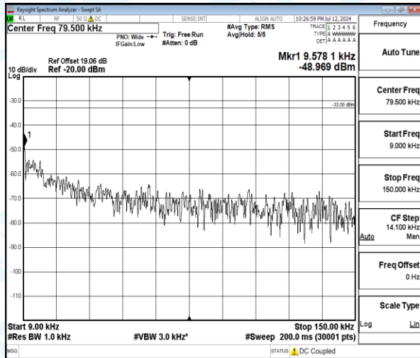
Band5-1.4MHz-16QAM-20525-1-0-Low-0.009-0.15-0.01--48.97-15.97--33-PASS
