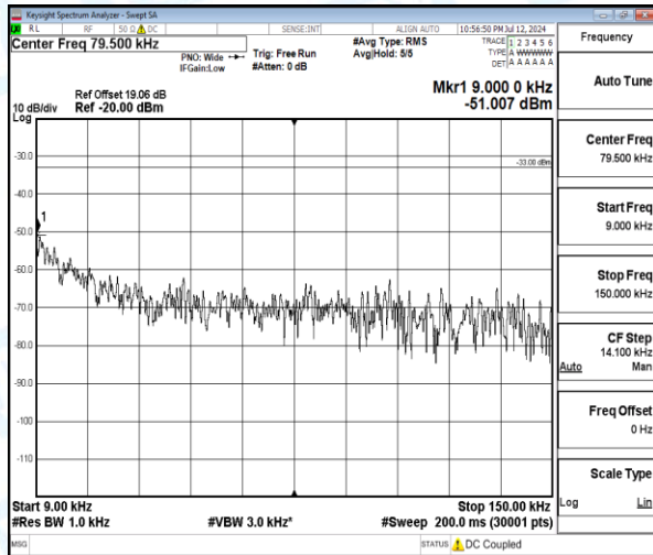
Band5-5MHz-16QAM-20525-1-0-Low-0.009-0.15-0.01--51.01-18.01--33-PASS
