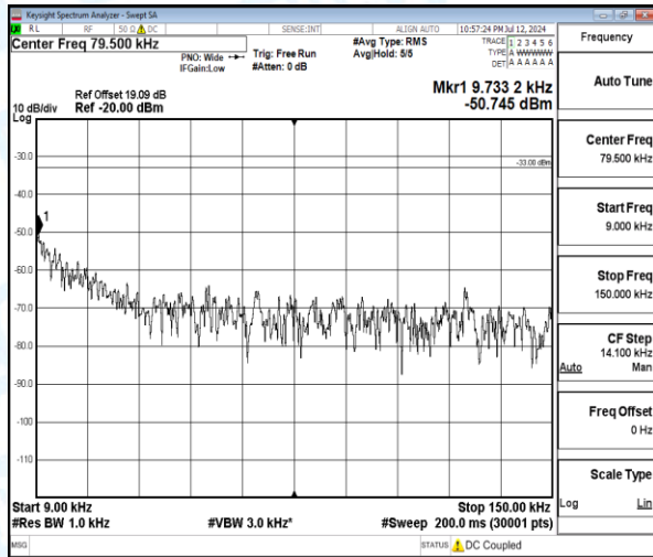
Band5-5MHz-QPSK-20625-1-0-High-0.009-0.15-0.01--50.75-17.75--33-PASS
