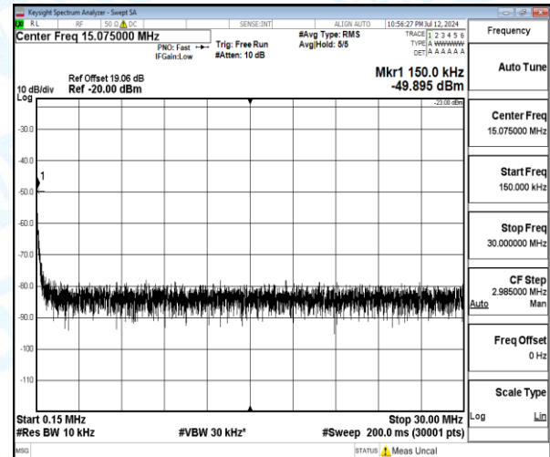
Band5-5MHz-QPSK-20525-1-0-Low-0.15-30-0.15--49.9-26.9--23-PASS
