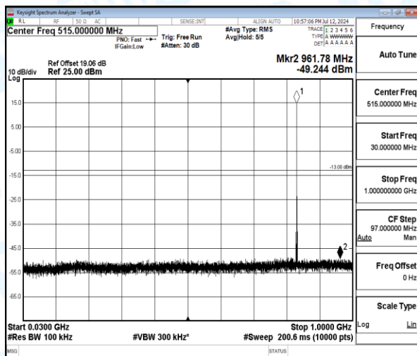
Band5-5MHz-16QAM-20525-1-0-Low-30-1000-961.78--49.24-36.24--13-PASS
