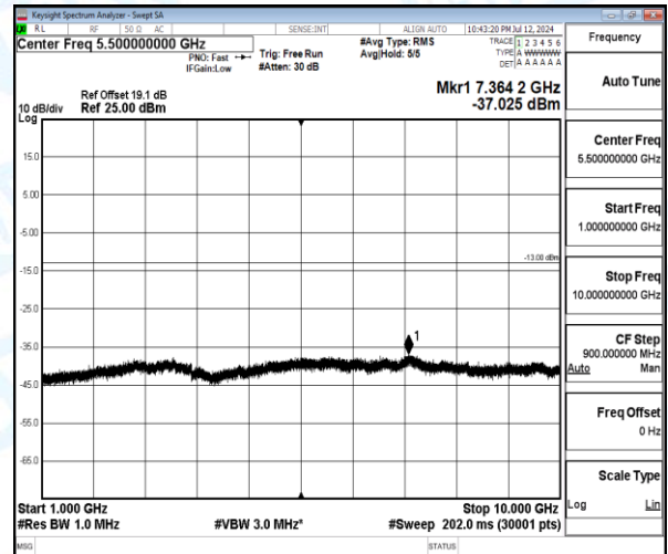
Band5-3MHz-16QAM-20635-1-0-High-1000-10000-7364.2--37.03-24.03--13-PASS
