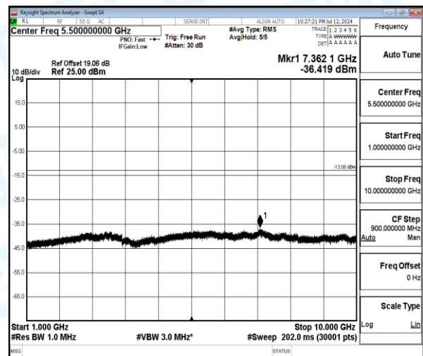
Band5-1.4MHz-16QAM-20525-1-0-Low-1000-10000-7362.1--36.42-23.42--13-PASS
