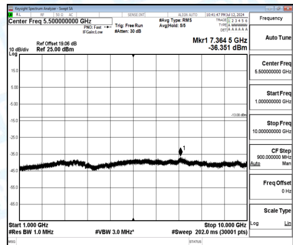
Band5-3MHz-QPSK-20525-1-0-Low-1000-10000-7364.5--36.35-23.35--13-PASS
