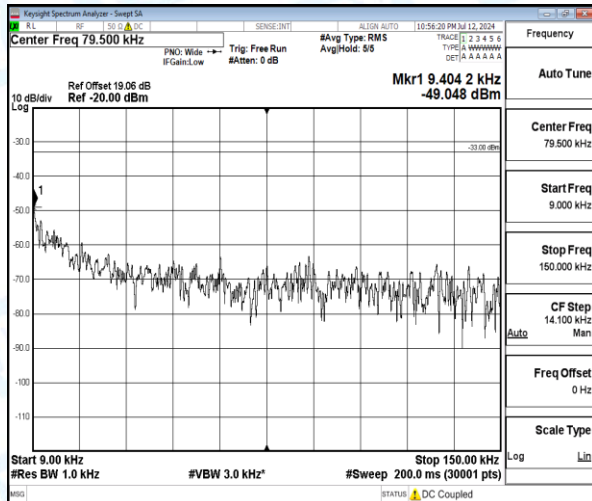
Band5-5MHz-QPSK-20525-1-0-Low-0.009-0.15-0.01--49.05-16.05--33-PASS
