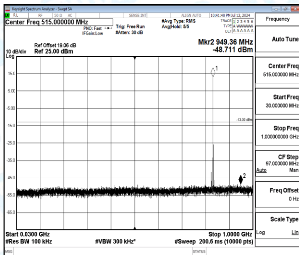
Band5-3MHz-QPSK-20525-1-0-Low-30-1000-949.36--48.71-35.71--13-PASS
