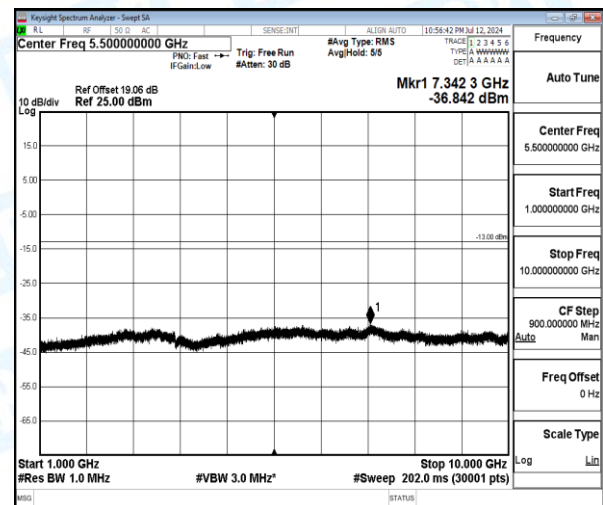
Band5-5MHz-QPSK-20525-1-0-Low-1000-10000-7342.3--36.84-23.84--13-PASS
