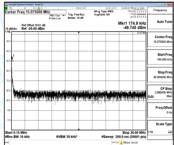
Band5-3MHz-QPSK-20415-1-0-Low-0.15-30-0.17--49.75-26.75--23-PASS
