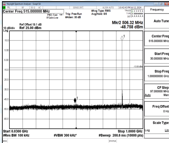
Band5-3MHz-QPSK-20635-1-0-High-30-1000-506.32--48.76-35.76--13-PASS
