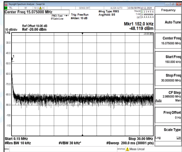
Band5-5MHz-16QAM-20525-1-0-Low-0.15-30-0.15--48.12-25.12--23-PASS
