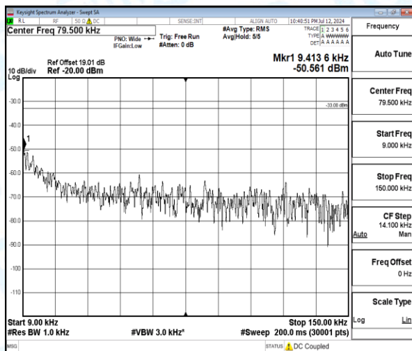
Band5-3MHz-16QAM-20415-1-0-Low-0.009-0.15-0.01--50.56-17.56--33-PASS
