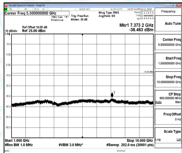
Band5-5MHz-16QAM-20525-1-0-Low-1000-10000-7373.2--36.46-23.46--13-PASS
