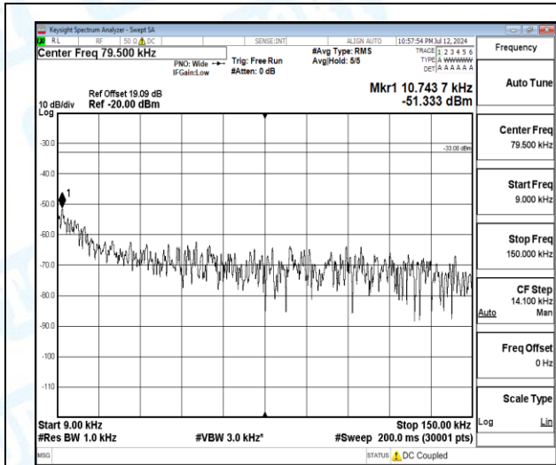
Band5-5MHz-16QAM-20625-1-0-High-0.009-0.15-0.01--51.33-18.33--33-PASS
