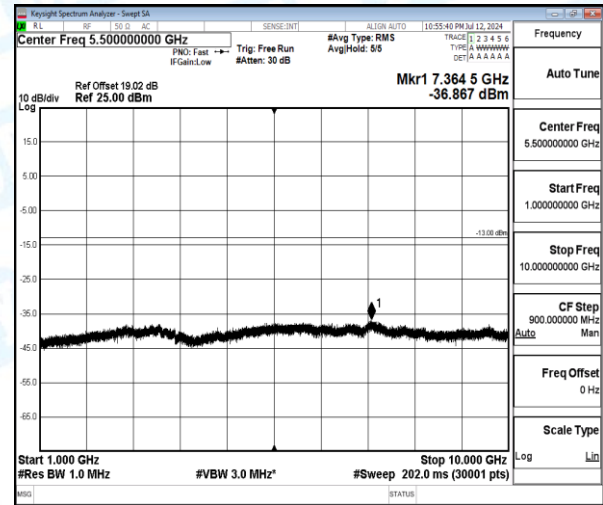
Band5-5MHz-QPSK-20425-1-0-Low-1000-10000-7364.5--36.87-23.87--13-PASS
