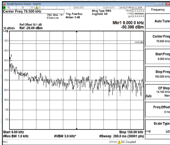
Band5-3MHz-QPSK-20635-1-0-High-0.009-0.15-0.01--50.4-17.4--33-PASS
