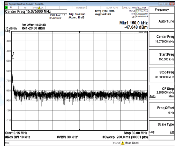
Band5-5MHz-QPSK-20625-1-0-High-0.15-30-0.15--47.65-24.65--23-PASS
