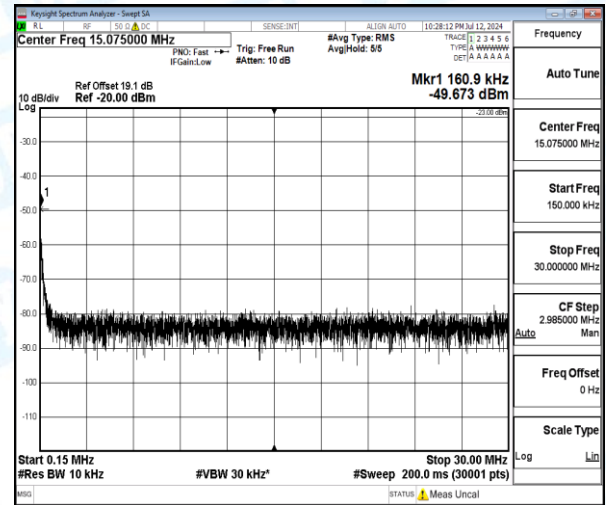
Band5-1.4MHz-16QAM-20643-1-0-High-0.15-30-0.16--49.67-26.67--23-PASS
