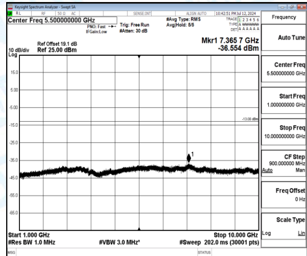
Band5-3MHz-QPSK-20635-1-0-High-1000-10000-7365.7--36.55-23.55--13-PASS
