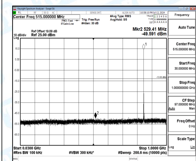
Band5-5MHz-16QAM-20625-1-0-High-30-1000-529.41--49.59-36.59--13-PASS
