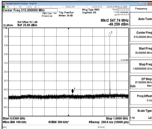
Band5-3MHz-16QAM-20635-1-0-High-30-1000-547.74--49.26-36.26--13-PASS
