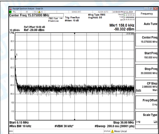
Band5-5MHz-16QAM-20625-1-0-High-0.15-30-0.16--50.33-27.33--23-PASS
