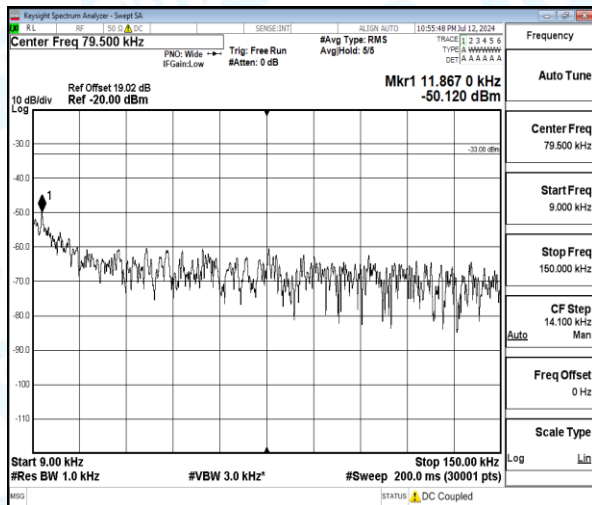
Band5-5MHz-16QAM-20425-1-0-Low-0.009-0.15-0.01--50.12-17.12--33-PASS
