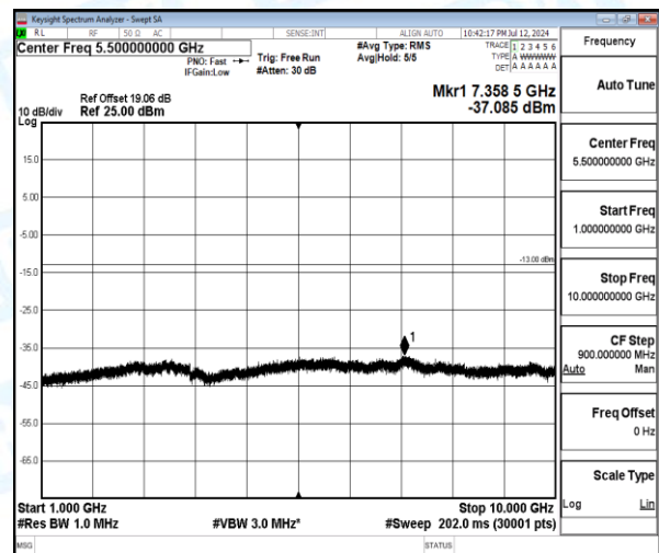
Band5-3MHz-16QAM-20525-1-0-Low-1000-10000-7358.5--37.09-24.09--13-PASS
