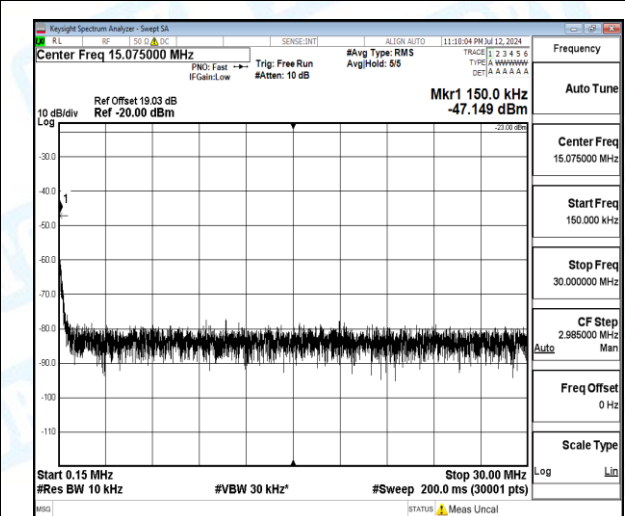
Band5-10MHz-QPSK-20450-1-0-Low-0.15-30-0.15--47.15-24.15--23-PASS
