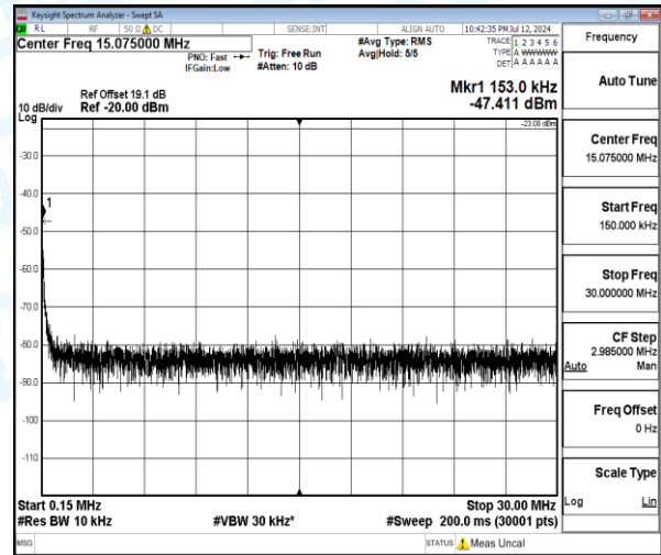
Band5-3MHz-QPSK-20635-1-0-High-0.15-30-0.15--47.41-24.41--23-PASS
