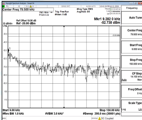
Band5-3MHz-QPSK-20525-1-0-Low-0.009-0.15-0.01--52.74-19.74--33-PASS
