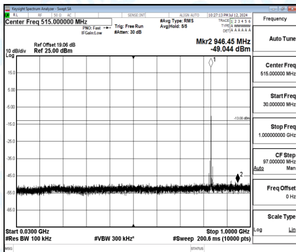
Band5-1.4MHz-16QAM-20525-1-0-Low-30-1000-946.45--49.04-36.04--13-PASS
