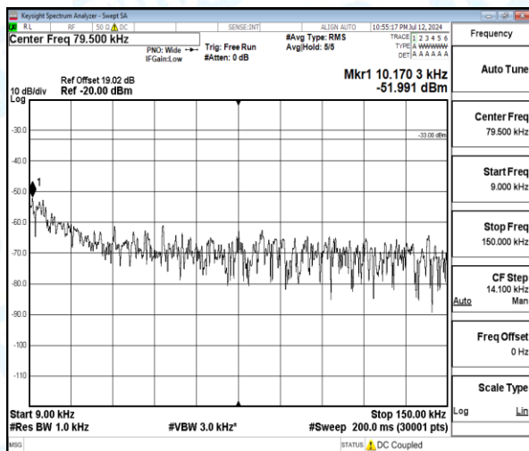
Band5-5MHz-QPSK-20425-1-0-Low-0.009-0.15-0.01--51.99-18.99--33-PASS
