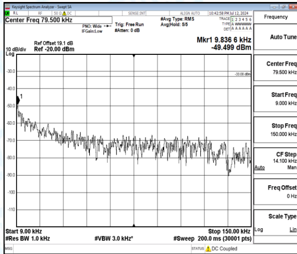
Band5-3MHz-16QAM-20635-1-0-High-0.009-0.15-0.01--49.5-16.5--33-PASS
