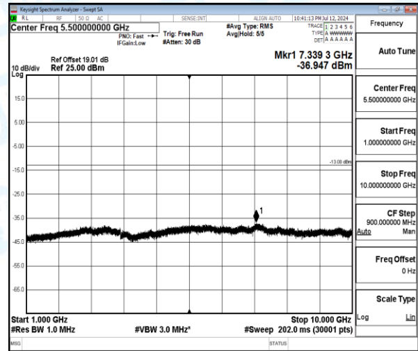
Band5-3MHz-16QAM-20415-1-0-Low-1000-10000-7339.3--36.95-23.95--13-PASS
