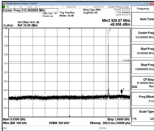
Band5-1.4MHz-16QAM-20407-1-0-Low-30-1000-929.67--48.96-35.96--13-PASS
