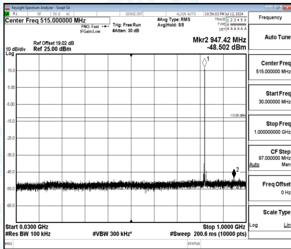
Band5-5MHz-16QAM-20425-1-0-Low-30-1000-947.42--48.5-35.5--13-PASS
