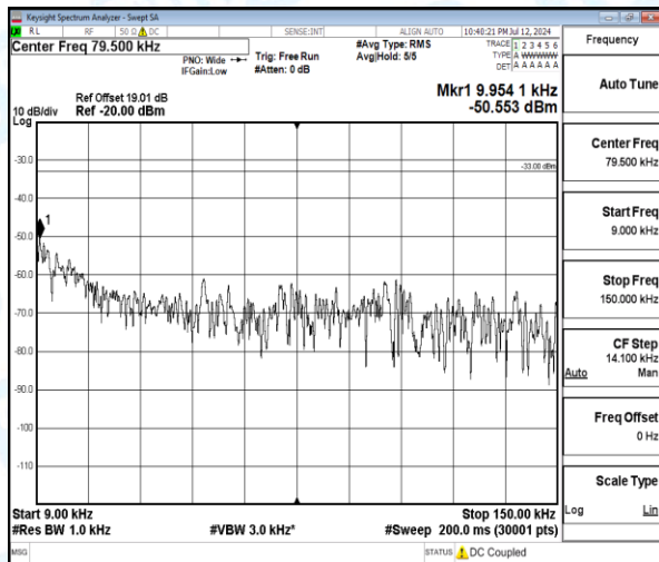
Band5-3MHz-QPSK-20415-1-0-Low-0.009-0.15-0.01--50.55-17.55--33-PASS
