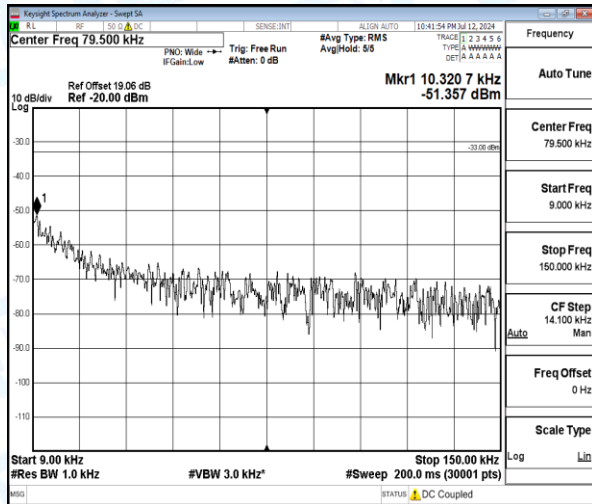
Band5-3MHz-16QAM-20525-1-0-Low-0.009-0.15-0.01--51.36-18.36--33-PASS
