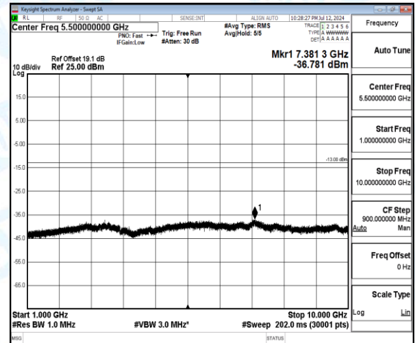
Band5-1.4MHz-16QAM-20643-1-0-High-1000-10000-7381.3--36.78-23.78--13-PASS
