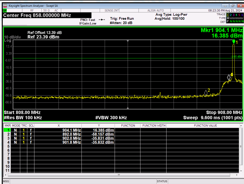
Band Edge NVNT LoRa 904MHz Ant1 Emission
