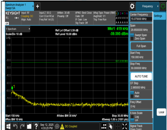
Band12-3MHz-QPSK-23025-1RB#14-1000~3000-PASS
