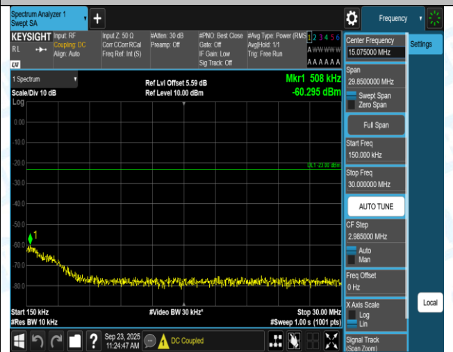
Band13-5MHz-QPSK-23255-25RB#0-1000~3000-PASS
