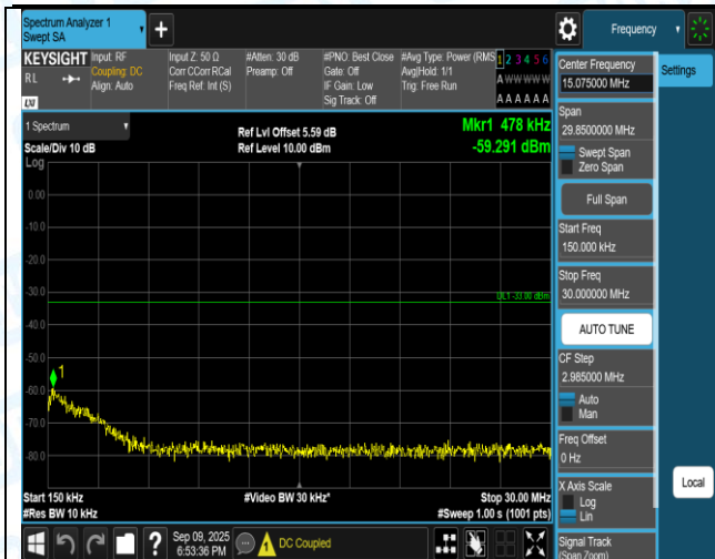
Band2-10MHz-16QAM-19150-1RB#0-1000~3000-PASS
