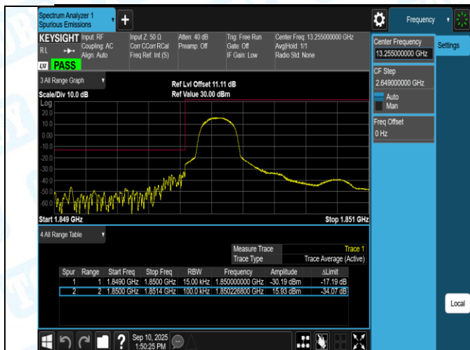
Band2-1.4MHz-16QAM-18607-6RB#0-PASS
