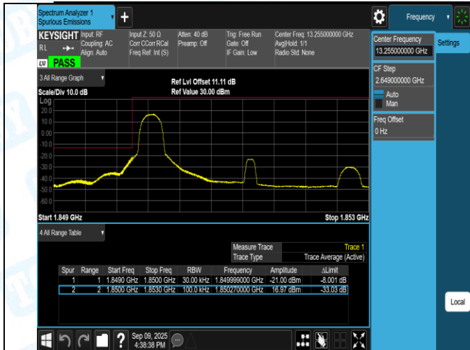
Band2-3MHz-16QAM-18615-15RB#0-PASS
