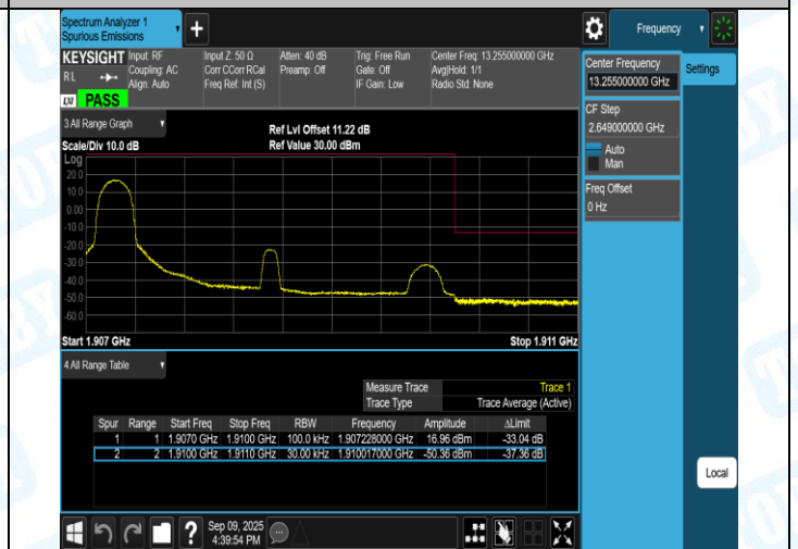
Band2-3MHz-QPSK-19185-15RB#0-PASS
