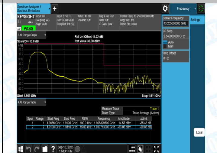
Band2-1.4MHz-16QAM-19193-6RB#0-PASS
