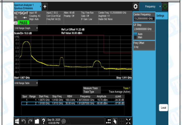
Band2-3MHz-16QAM-19185-15RB#0-PASS
