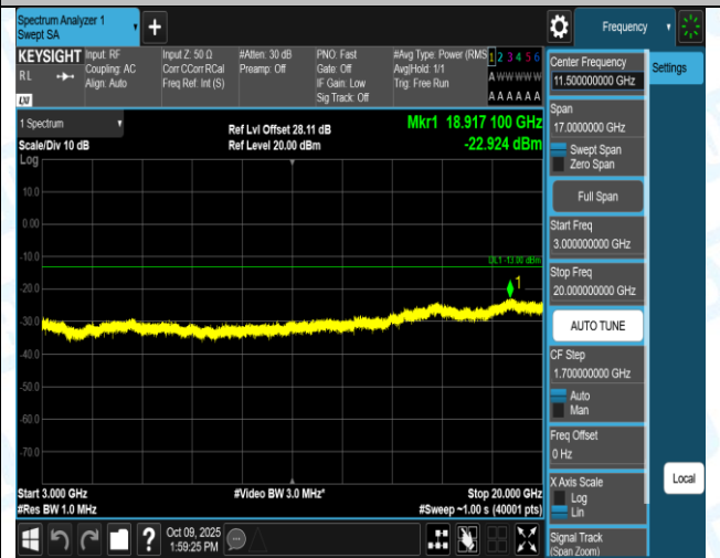
Band2-1.4MHz-QPSK-18607-6RB#0-0.15~30-PASS
