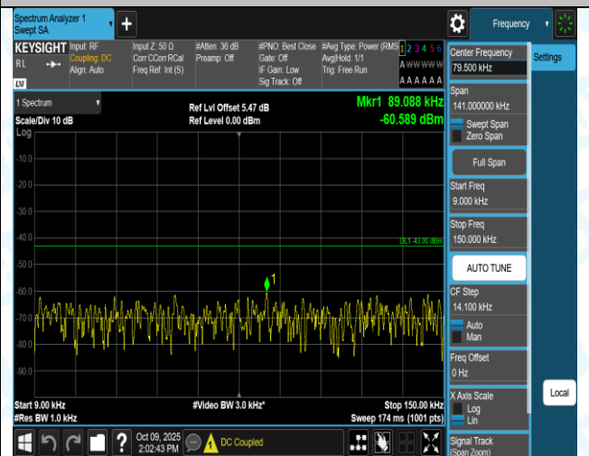
Band2-1.4MHz-QPSK-18900-1RB#0-30~1000-PASS
