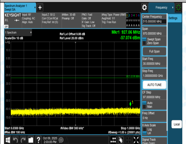
Band2-1.4MHz-QPSK-18900-1RB#0-3000~20000-PASS
