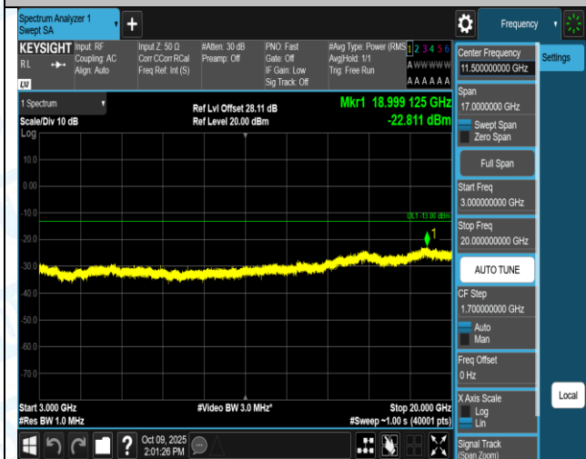
Band2-1.4MHz-QPSK-18900-1RB#0-0.15~30-PASS
