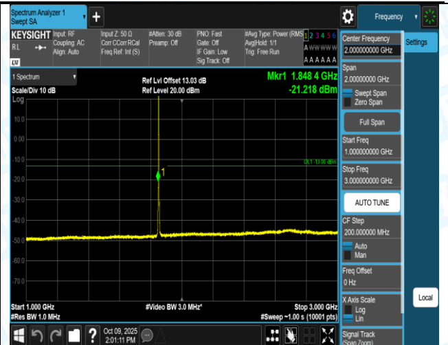
Band2-1.4MHz-QPSK-18900-1RB#0-0.009~0.15-PASS
