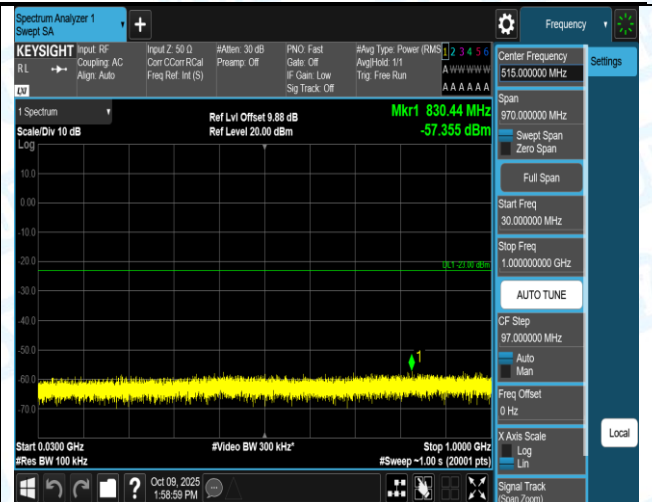
Band2-1.4MHz-QPSK-18607-1RB#5-3000~20000-PASS
