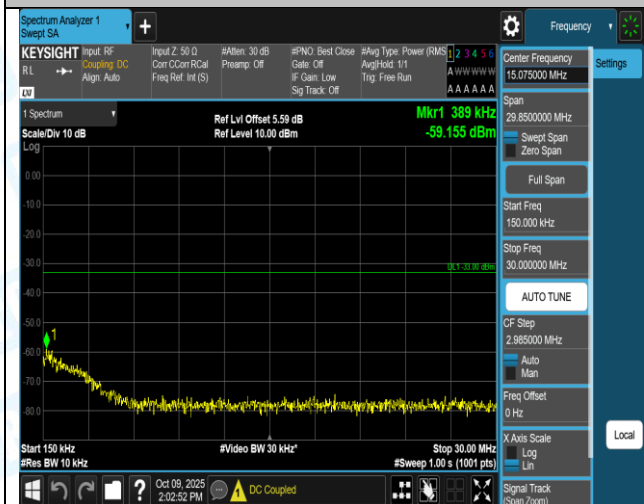
Band2-1.4MHz-QPSK-18900-1RB#0-1000~3000-PASS
