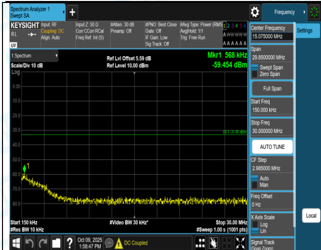
Band2-1.4MHz-QPSK-18607-1RB#5-1000~3000-PASS
