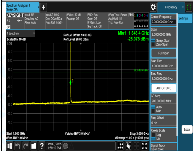
Band2-1.4MHz-QPSK-18607-6RB#0-0.009~0.15-PASS
