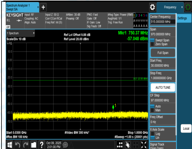
Band2-1.4MHz-QPSK-18607-6RB#0-3000~20000-PASS
