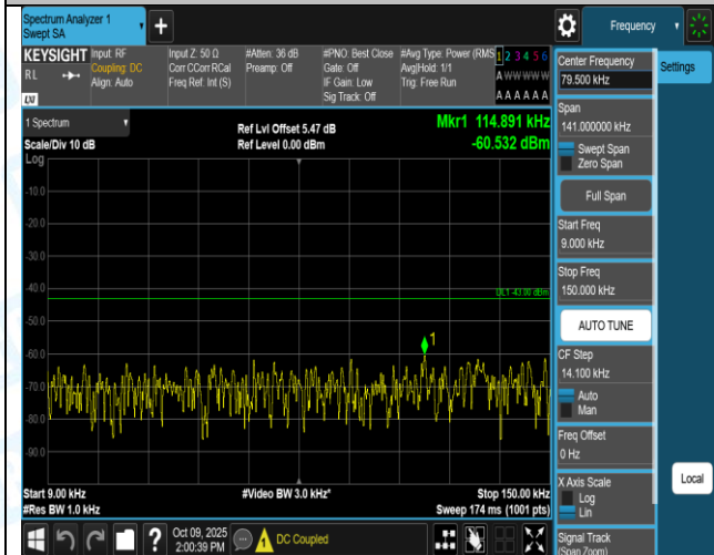
Band2-1.4MHz-QPSK-18607-6RB#0-30~1000-PASS
