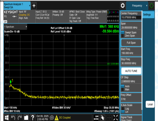
Band2-1.4MHz-QPSK-18607-6RB#0-1000~3000-PASS
