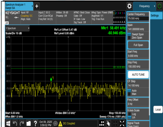
Band2-1.4MHz-QPSK-19193-1RB#0-30~1000-PASS
