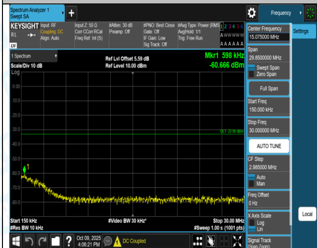
Band2-3MHz-16QAM-18615-1RB#0-1000~3000-PASS
