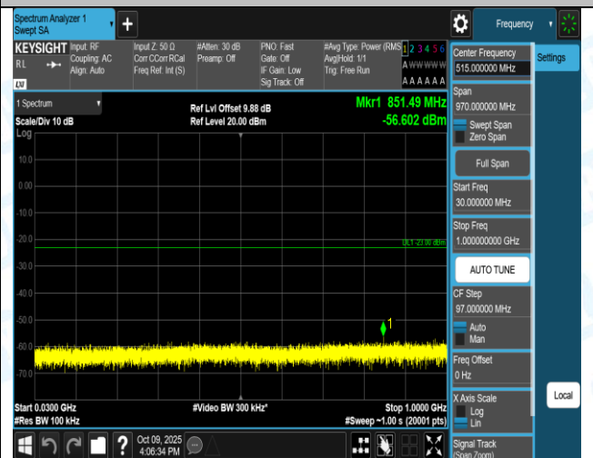
Band2-3MHz-16QAM-18615-1RB#0-3000~20000-PASS
