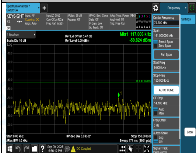
Band2-10MHz-QPSK-18650-50RB#0-30~1000-PASS
