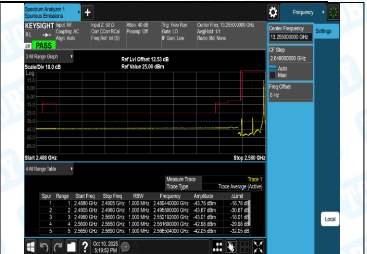
Band38-10MHz-16QAM-38200-1RB#49-PASS
