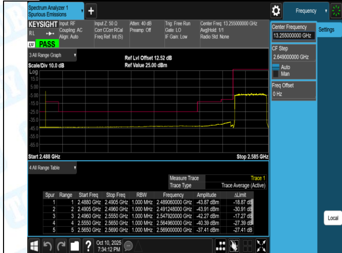
Band38-15MHz-QPSK-38175-1RB#74-PASS
