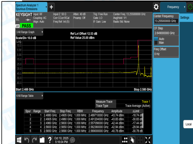
Band38-10MHz-16QAM-38200-1RB#0-PASS
