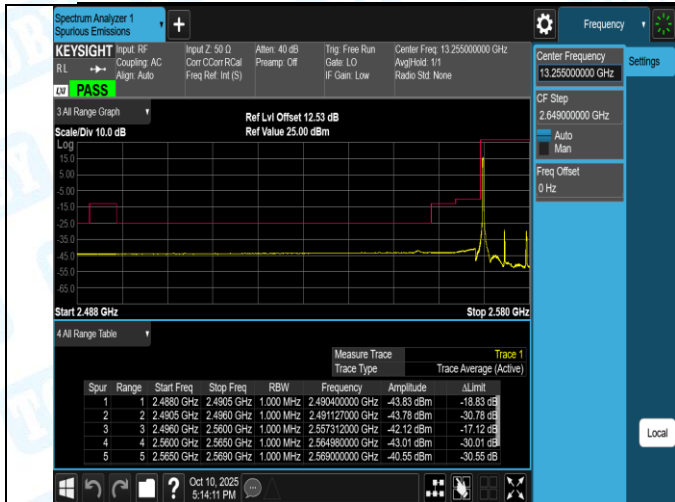
Band38-10MHz-QPSK-37800-50RB#0-PASS
