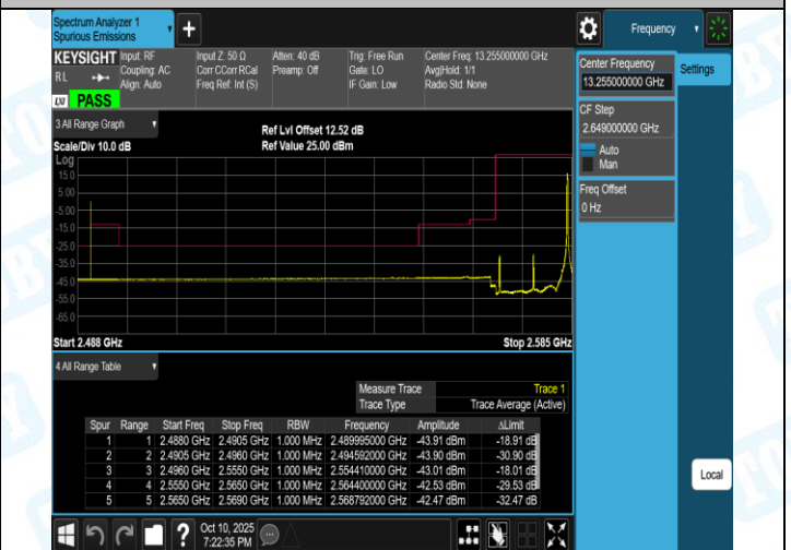
Band38-15MHz-QPSK-38175-1RB#0-PASS
