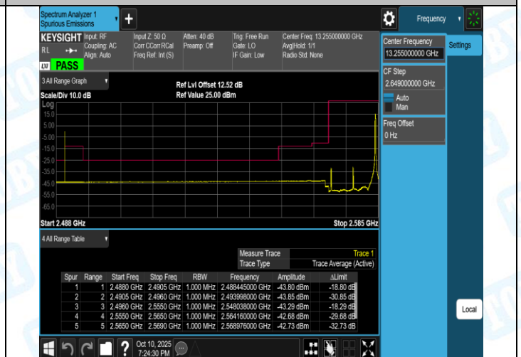
Band38-15MHz-16QAM-38175-1RB#74-PASS
