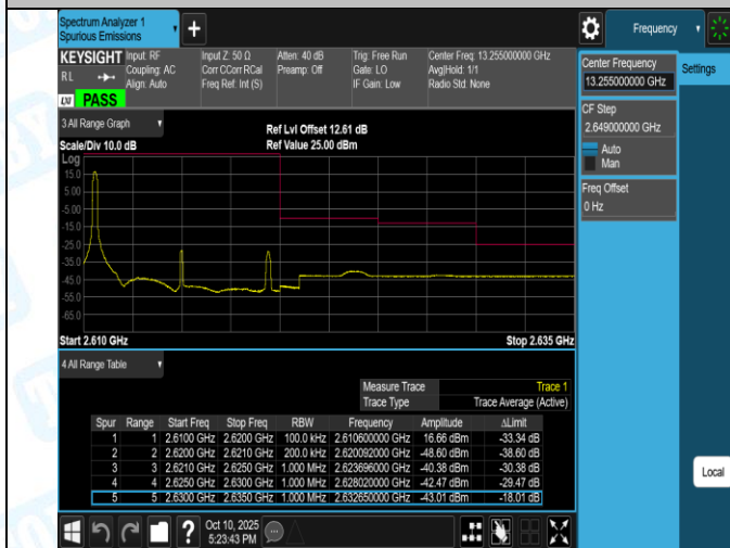
Band38-15MHz-QPSK-37825-1RB#0-PASS
