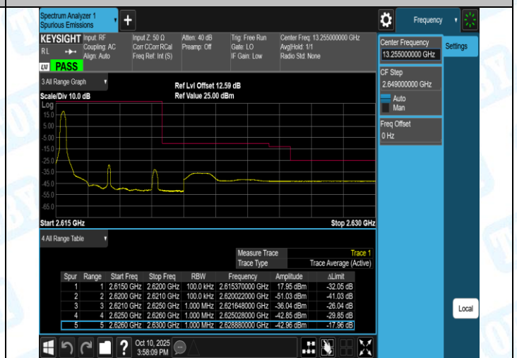
Band38-5MHz-16QAM-38225-25RB#0-PASS
