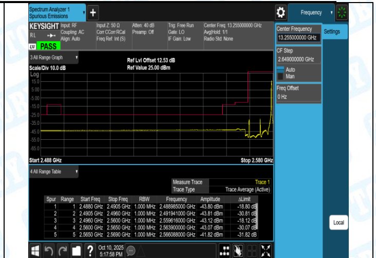
Band38-10MHz-QPSK-38200-1RB#0-PASS
