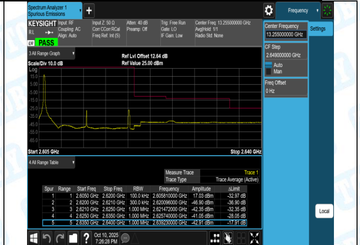
Band38-15MHz-QPSK-38175-75RB#0-PASS
