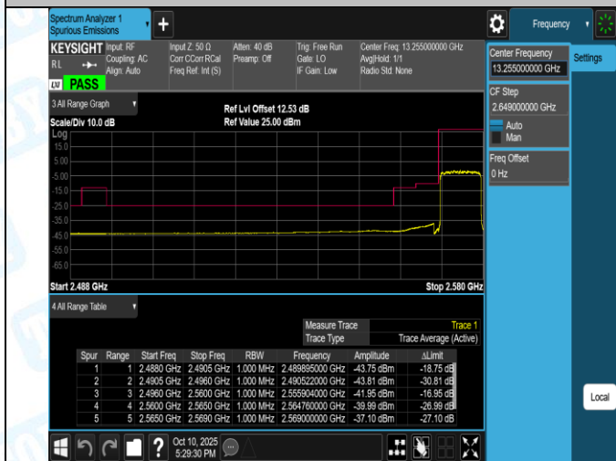
Band38-10MHz-QPSK-38200-1RB#49-PASS
