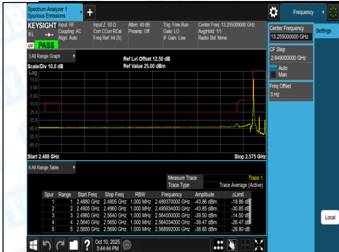
Band38-5MHz-16QAM-37775-25RB#0-PASS
