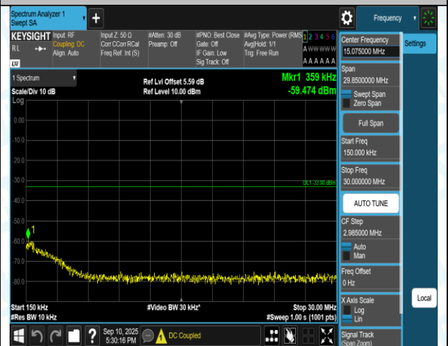
Band4-5MHz-16QAM-20375-1RB#24-1000~3000-PASS
