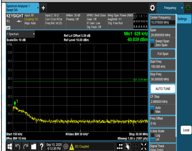
Band4-10MHz-16QAM-20175-1RB#0-1000~3000-PASS
