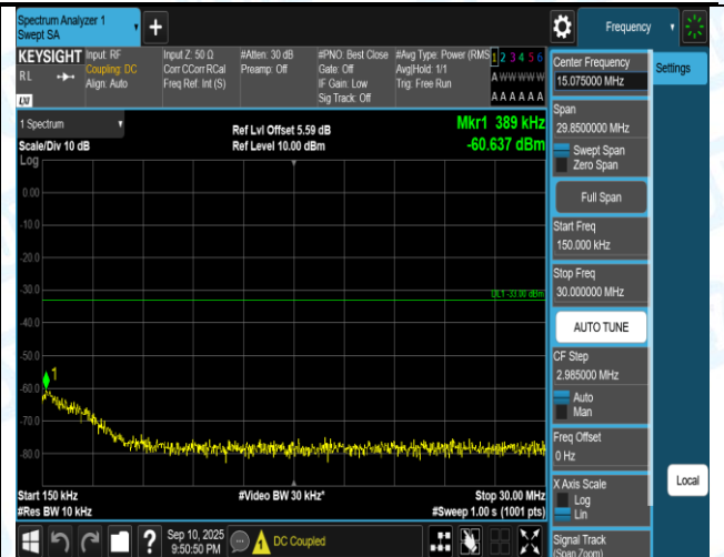
Band4-15MHz-16QAM-20025-1RB#0-1000~3000-PASS
