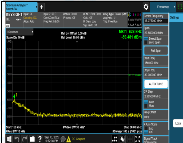
Band4-15MHz-16QAM-20025-1RB#74-1000~3000-PASS
