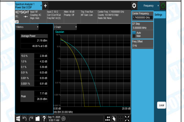
Band4-20MHz-QPSK-20300-100RB#0-PASS
