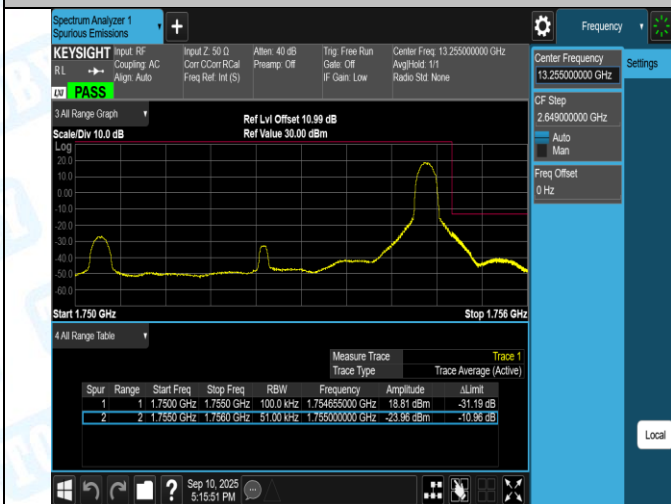
Band4-5MHz-16QAM-19975-1RB#0-PASS
