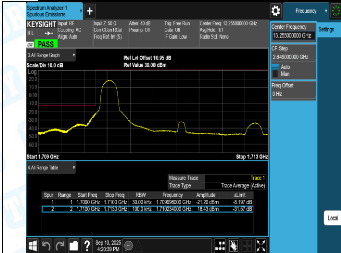
Band4-3MHz-QPSK-19965-15RB#0-PASS
