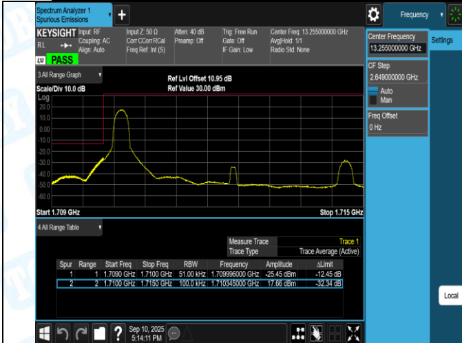
Band4-5MHz-16QAM-19975-25RB#0-PASS
