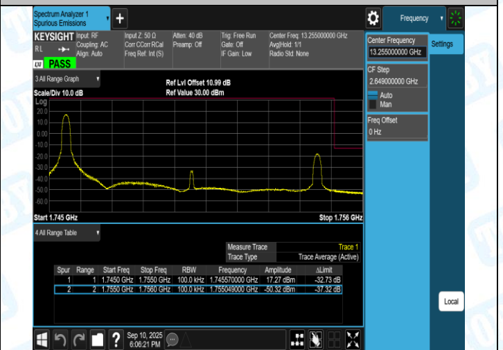
Band4-10MHz-QPSK-20350-50RB#0-PASS
