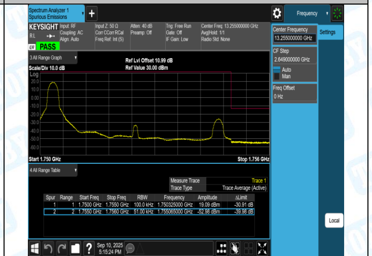
Band4-5MHz-QPSK-20375-25RB#0-PASS
