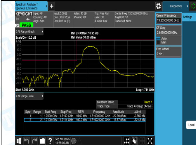
Band4-1.4MHz-16QAM-19957-6RB#0-PASS
