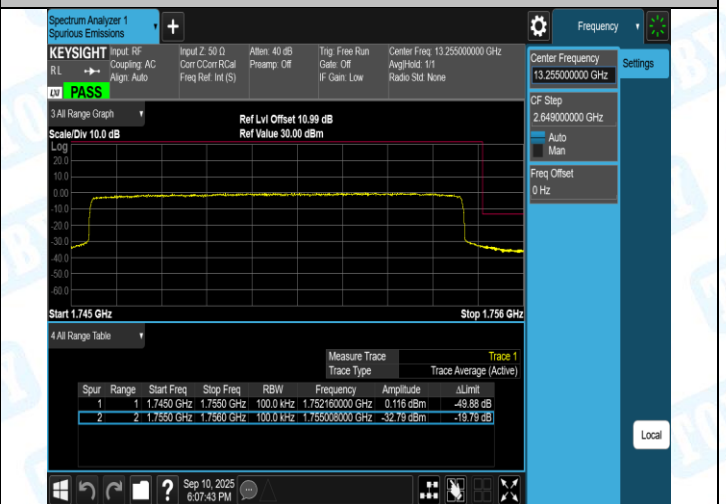
Band4-10MHz-16QAM-20000-1RB#49-PASS
