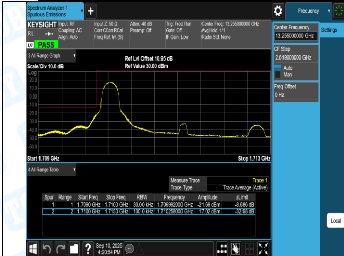
Band4-3MHz-16QAM-19965-15RB#0-PASS
