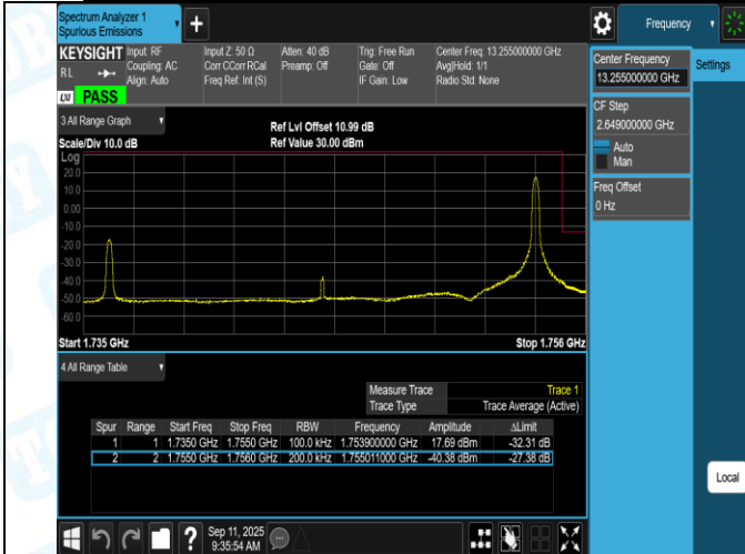
Band4-20MHz-16QAM-20050-1RB#0-PASS
