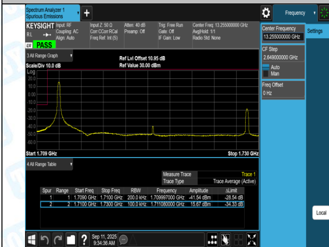
Band4-20MHz-16QAM-20300-1RB#0-PASS
