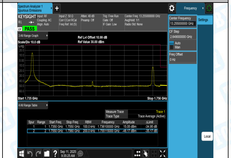
Band4-20MHz-QPSK-20300-100RB#0-PASS
