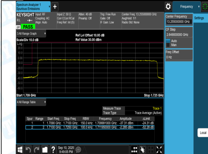
Band4-15MHz-QPSK-20325-1RB#74-PASS
