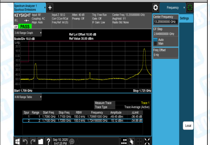
Band4-15MHz-QPSK-20325-1RB#0-PASS
