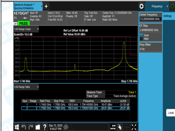
Band4-15MHz-16QAM-20025-1RB#0-PASS
