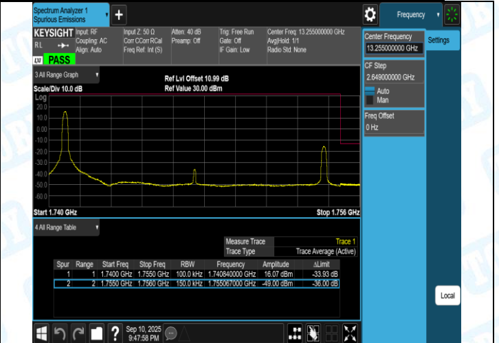
Band4-15MHz-QPSK-20325-75RB#0-PASS
