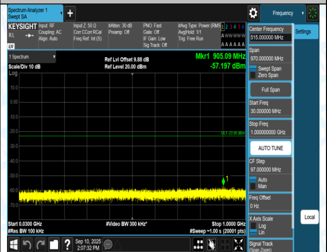
Band4-1.4MHz-16QAM-19957-6RB#0-3000~20000-PASS
