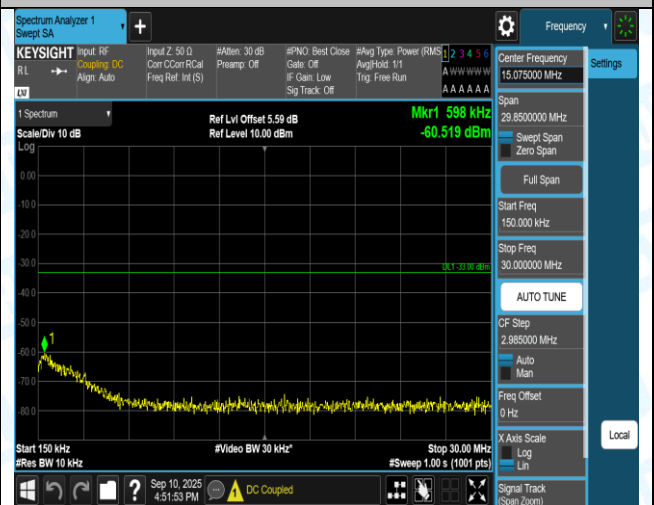
Band4-3MHz-16QAM-20385-1RB#14-1000~3000-PASS
