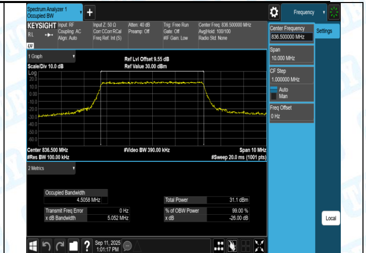
Band5-5MHz-16QAM-20425-25RB#0-PASS
