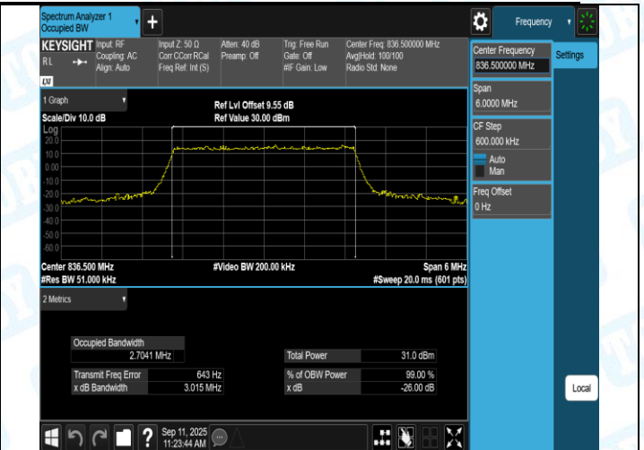
Band5-3MHz-16QAM-20415-15RB#0-PASS
