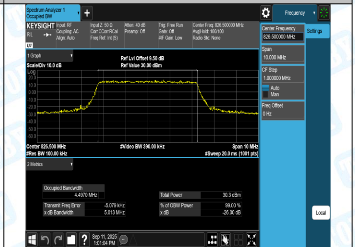
Band5-5MHz-16QAM-20625-25RB#0-PASS
