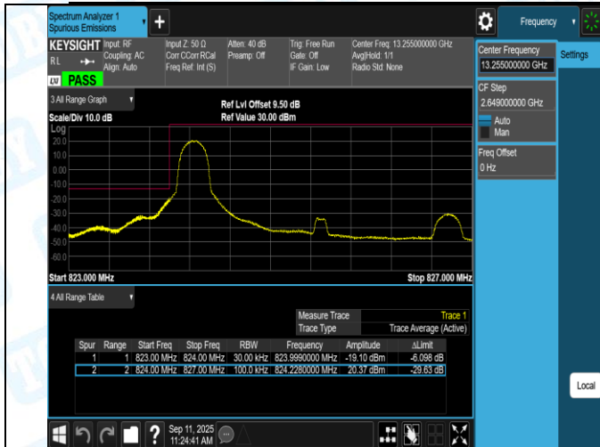
Band5-3MHz-QPSK-20415-15RB#0-PASS
