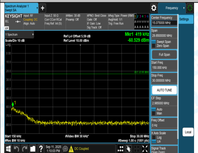
Band5-5MHz-QPSK-20425-25RB#0-1000~3000-PASS
