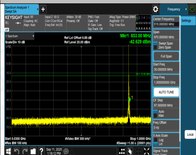
Band5-5MHz-16QAM-20625-1RB#0-3000~10000-PASS
