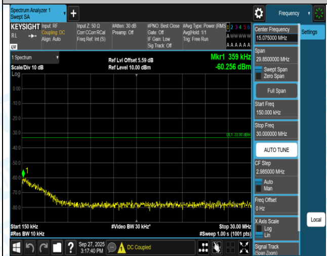
Band66-10MHz-16QAM-132322-1RB#0-1000~3000-PASS
