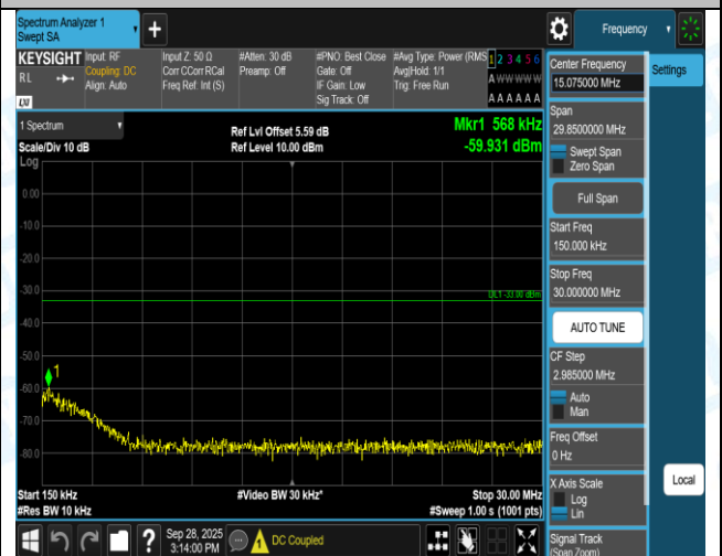
Band66-15MHz-QPSK-132322-75RB#0-1000~3000-PASS
