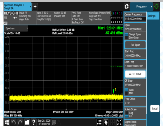
Band66-15MHz-QPSK-132047-75RB#0-30~1000-PASS
