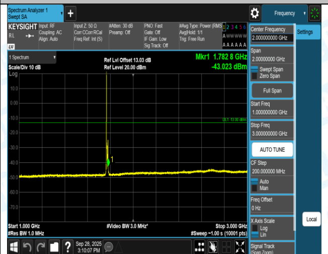
Band66-15MHz-16QAM-132597-1RB#74-0.009-0.15-PASS
