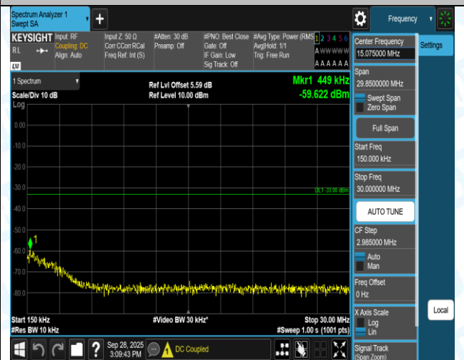
Band66-15MHz-16QAM-132597-1RB#0-1000~3000-PASS
