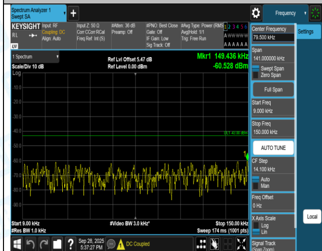
Band66-20MHz-QPSK-132572-100RB#0-30~1000-PASS
